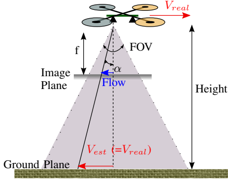
Fig. 3: Velocity estimation by measuring optical flow with one camera and height with both cameras of the stereo-camera.
