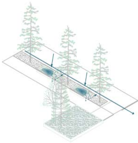
Domain 2: pipe system, detention basin, overflow/bypassing in bioretention
