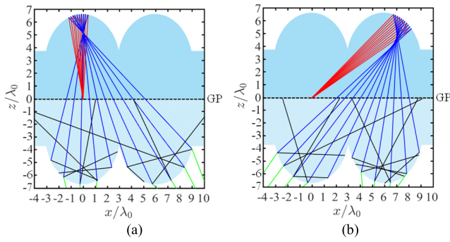
Fig. 9. Ray-tracing pictures corresponding to secondary reflections via the ground plane originating from (a) fed lens, and (b) neighboring lens when lens array is along the x -axis (H-plane). The red, blue, black, and green colored rays correspond to incidence, primary, secondary reflections, and transmission at the lens surfaces, respectively. A y -polarized CWG is located at the lower focus of the fed (left side) lens.
