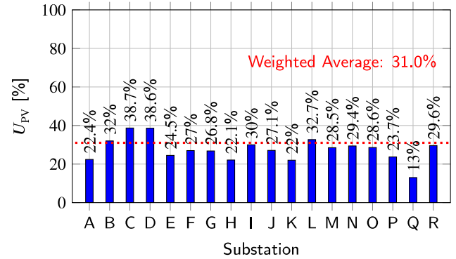
Fig. 9. PV Utilization ( U_{\text{PV}} ) at each substation in Arnhem for scenario 1: the decentralized energy-neutral approach without storage.
