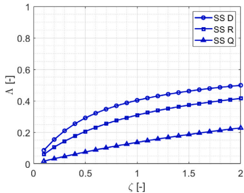
Fig. 11. Direct load coverage, \Lambda , for three substations in Arnhem: Largest (SS-D), average (SS-R), and smallest (SS-Q).
