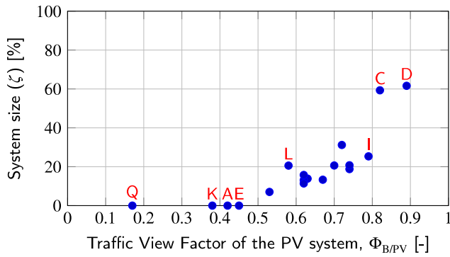
Fig. 14. PV system size as a fraction of the Energy Neutral size for each substation versus the traffic view factor of the PV system \Phi_{B/PV} .
