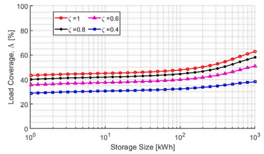
Fig. 15. Direct load coverage, \Lambda , for different \zeta values and storage sizes for the large substation D.
