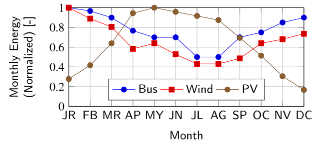
Fig. 4. Yearly simulated bus demand, wind generation, and PV generation trends by month for the entire Arnhem grid. Each variable is normalized with respect to the highest monthly value it reports. It is observable that the wind generation better follows the bus demand trend on a yearly basis.
