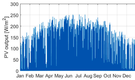
Fig. 7. Output of the yearly simulated PV generation in Arnhem in W/m2.
