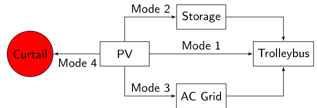
Fig. 3. The PV power flow: Generated energy can be used directly by the trolleybus (mode 1, most desirable), kept in the storage for later use by the trolleybus (mode 2), sent to the AC Grid – if local policy allows it – to be used later by the trolleybus (mode 3, net metering), or curtailed (mode 4, wasted).
