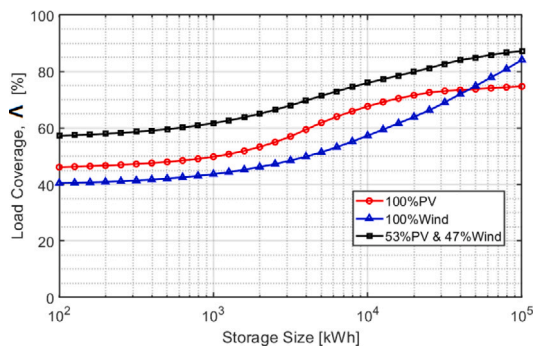
Fig. 19. Direct Load coverage as a function of the hybrid RES system composition (PV and Wind) with storage.
