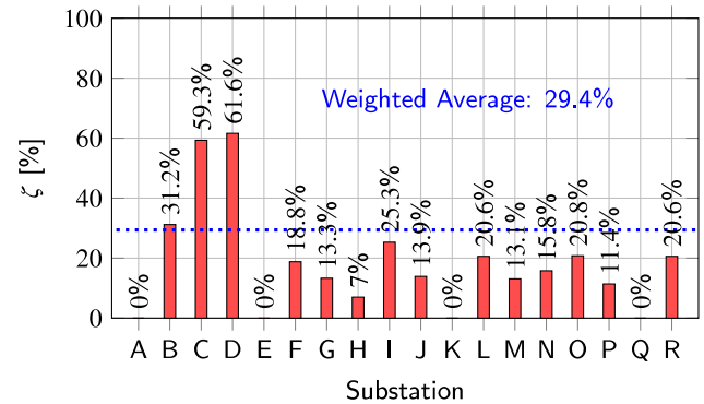
Fig. 13. Attainable fraction of energy neutral sizing for each substation using the Marginal Utilization Sizing approach. For substations A, E, K, and Q, no PV is advised.
