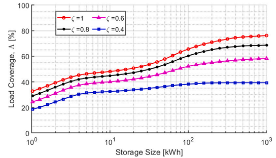
Fig. 16. Direct load coverage, \Lambda , for different \zeta values and storage sizes for the small substation Q.
