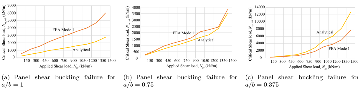
Figure 11. Validation results for panel shear buckling
