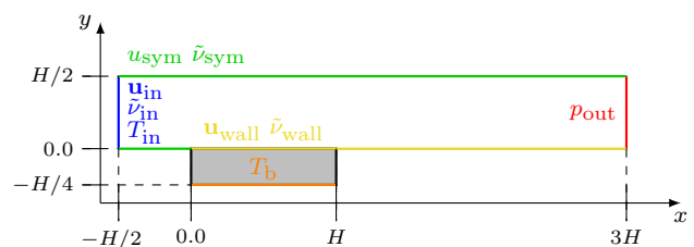
Fig. 9 Turbulent flow over a thick flat plate with a prescribed temperature at its bottom side: geometry and boundary conditions
