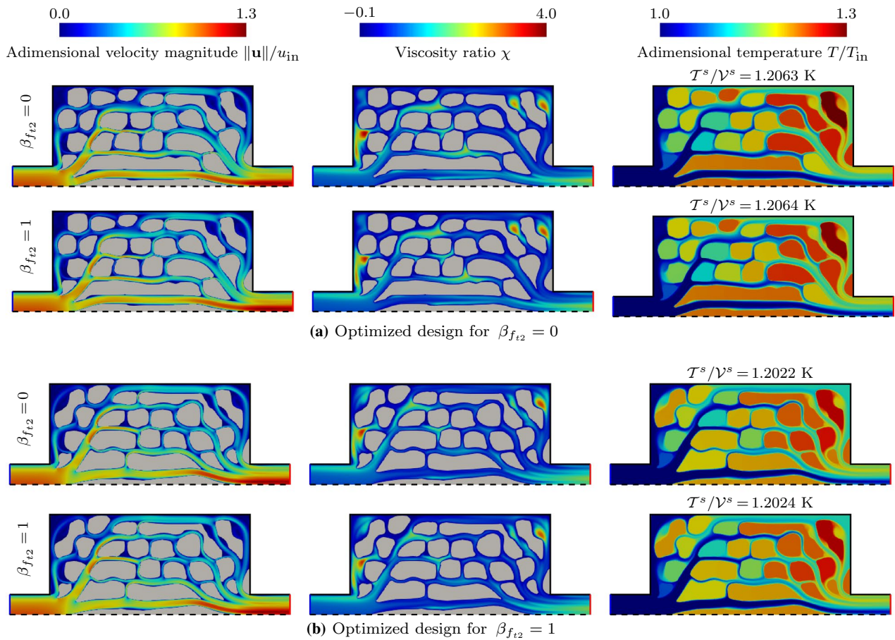
Fig. 19 Heat exchanger with a single outlet: optimized designs and performance in terms of average temperature in the solid domain T/\mathcal{V}^s for a Reynolds number Re = 5000 , at a fixed power dissipation with w_d = 0.33
