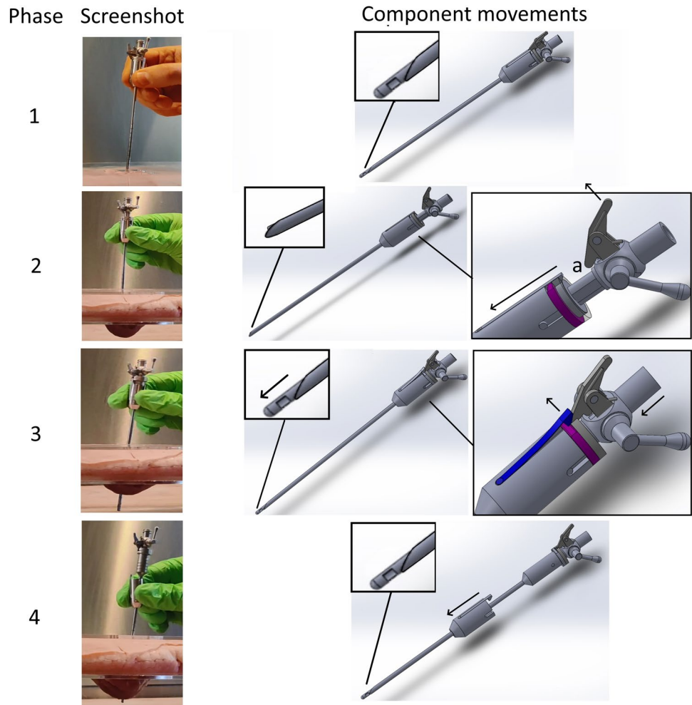
Fig. 4 Basic functioning of the VN+ design. Phase 1, the rest situation where the system is ready for use. Phase 2, during insertion the sharp cannula is exposed and the decoupling mechanism is armed automatically. Phase 3, as soon as the cannula tip penetrates the last tissue layer the stylet shoots out and decouples the grip component when the lever finger lifts the hook (dark blue) over the fixation ring (magenta). Phase 4, the force exerted by the hand on the needle is instantly decoupled resulting in acceleration of the grip component opposite to the housing (Color figure online)
