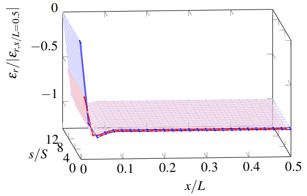
(b) (12,12) armchair
