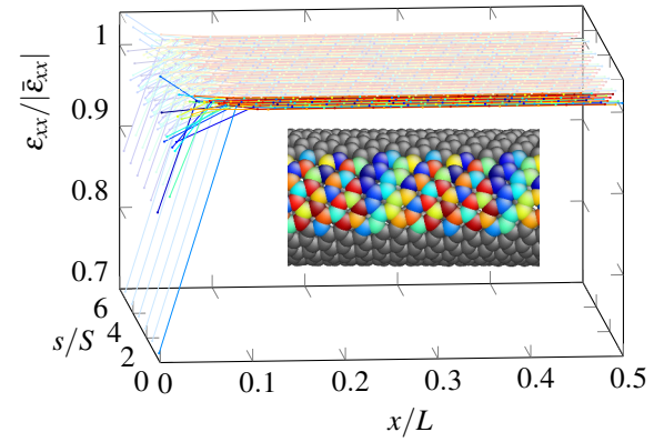
(e) (18,6) chiral
