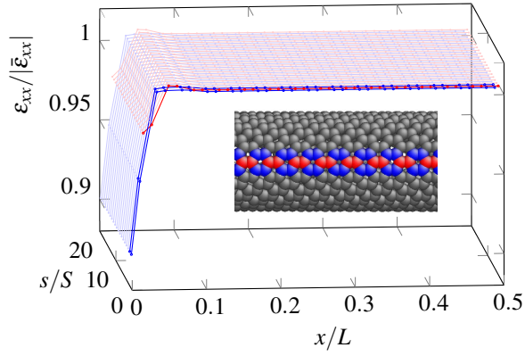
(c) (20,0) zigzag
