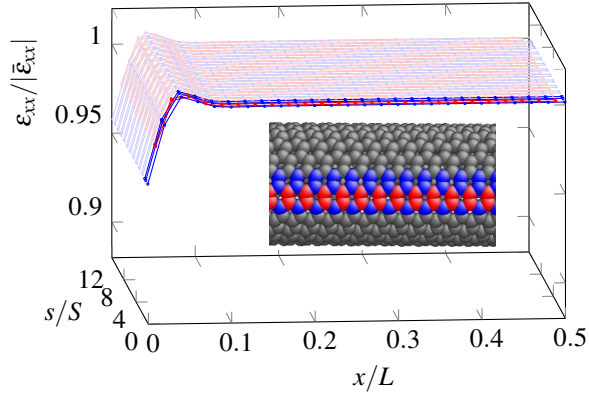
(a) (12,12) armchair
