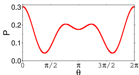
Figure 8. The power of the illuminating wavefield is defined by a_0 = 1/2\pi , a_2 = 1/4\pi and a_3 = 1/5\pi . The cross-spectra resulting from such an illumination pattern are shown in Fig. 9.
