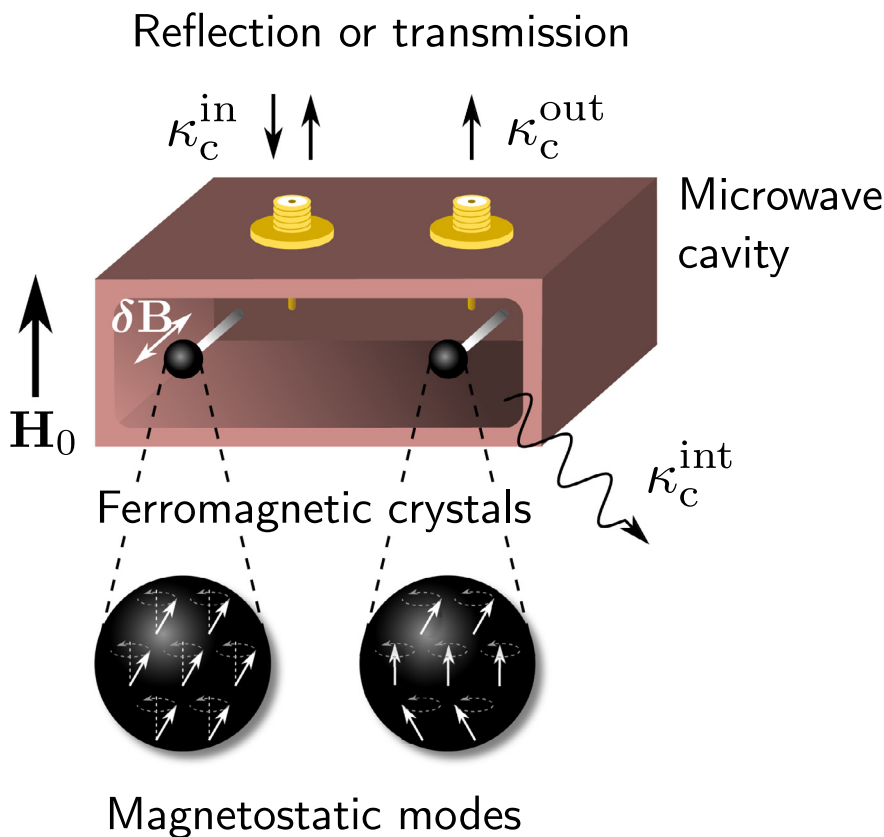
Fig. 10. Schematic diagram of a general hybrid system for creating cavity–magnon polaritons. The vacuum fluctuations \delta \mathbf{B} of the MW magnetic field of a cavity mode overlaps with one or more ferromagnetic crystals. An external magnetic field \mathbf{H}_0 = \mathbf{B}_0/\mu_0 is applied either uniformly or locally to each magnet. Depending on the uniformity of the MW magnetic field of the cavity mode, different magnetostatic modes can be coupled. The MW cavity can be probed either by transmission or reflection through coupling rates \kappa_c^{\text{in}} and \kappa_c^{\text{out}} to input and output ports. The internal loss of the MW cavity mode is given by \kappa_c^{\text{int}} .
