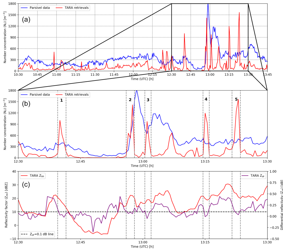
Figure 9. Time series of the N_T retrievals: (a) zoomed version for the period between 12:30 and 13:30 UTC (b) and the corresponding Z_{hh} and Z_{dr} observations from the disdrometer and the radar (c).
