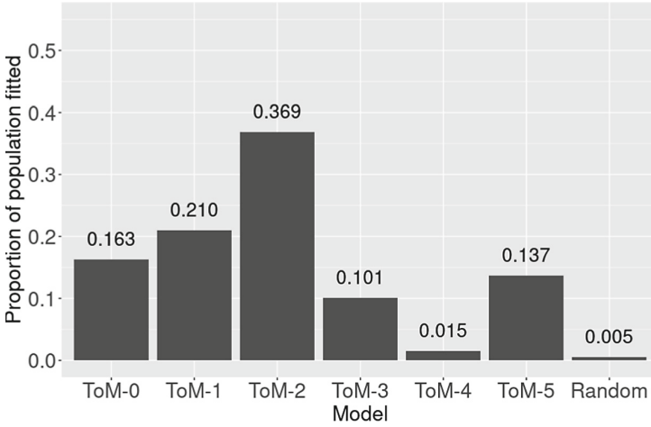
Fig. 4. Relative frequencies of each ToM level and the random model as predicted by RFX-BMS, for the data of [8], using ToM models.
