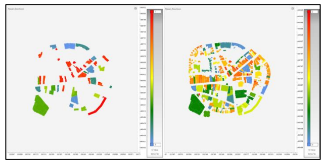
Figure 6. Comparison of the output of the PhysicsPreprocessor step using the different Dutch (left) and German (right) physics libraries.
