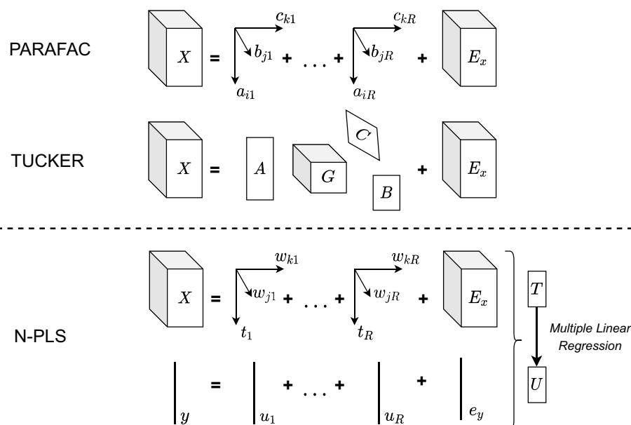
FIGURE 6 Schematization of multi-way models. The cubes (cuboids) represent three dimensional arrays ( X denoting the data array, G the core-array for the Tucker model and E_x the residual array for all models), the three arrows represent orthogonal vectors (trilinear factors a_1 , b_1 , c_1 , and loading vectors w_k , w_j with score vector t ), while the lines represent vectors (response vector y , score vector u , and residual vector e_y ), and the rectangles represent loading matrices for the Tucker model ( A , B , C ). Adopted from (Fujiwara and Mohr, 2009).
