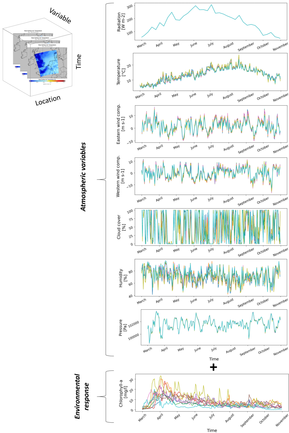
FIGURE 4 Illustration of the atmospheric and environmental variables used in the study.
