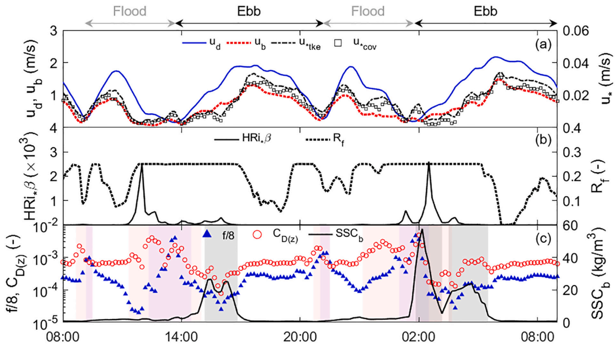
Fig. 7. Time series of (a) depth-averaged velocity ( u_d ), near-bed velocity ( u_b ) and friction velocity given by the TKE method ( u_{*tke} ) and COV method ( u_{*cov} ), (b) near-bed flux Richardson number ( R_f ) and the term H Ri_* \beta where H is the water depth, Ri_* is bulk Richardson number and \beta is Rouse number, and (c) near-bed suspended sediment concentration ( SSC_b ), friction coefficient ( f ) and drag coefficient ( C_{D(z)} ). The red and blue shadings indicate the periods when u_b and u_d are less than 0.5 m/s, respectively. The presence of concentrated benthic suspensions corresponds to grey shading. (For interpretation of the references to colour in this figure legend, the reader is referred to the web version of this article.)
