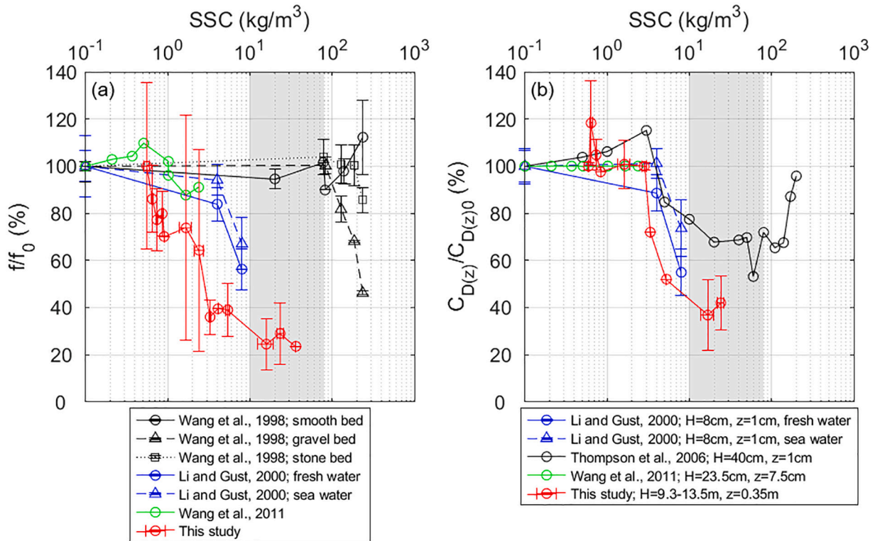
Fig. 8. Normalized (a) friction coefficient ( f/f_0 ) and (b) drag coefficient ( C_{D(z)}/C_{D(z)_0} ) versus suspended sediment concentration (SSC). The symbols f_0 and C_{D(z)_0} denote the friction coefficient and drag coefficient within the observed lowest SSC. Various types of scatter points represent data from laboratory experiments reported in the literature and field observations (this study). The SSC range of concentrated benthic suspension corresponds to grey shading (Wang et al., 2011).
