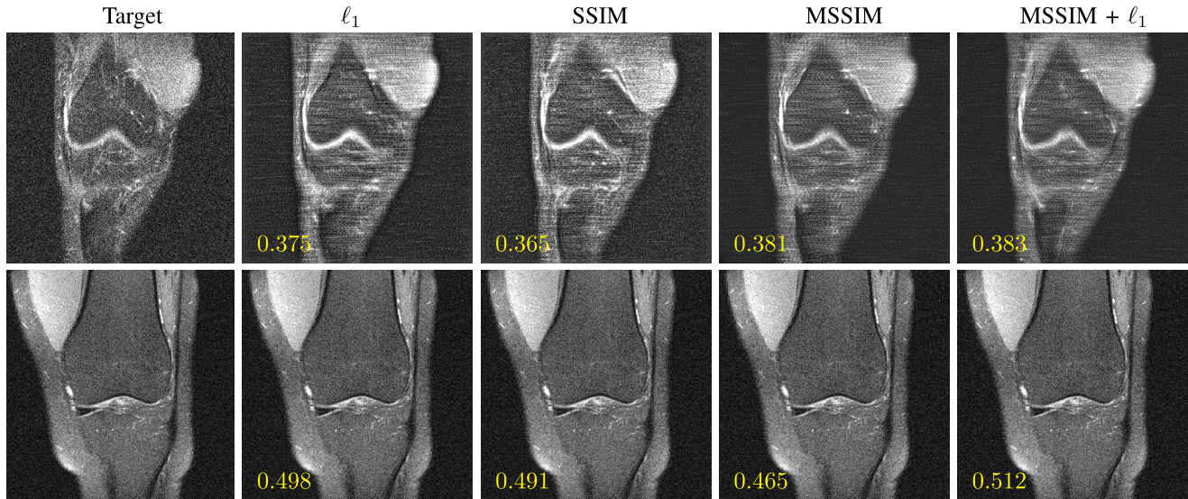
FIGURE 3. Two examples of single-coil 4\times for the different loss functions. A small network is used to test several losses. SSIM values are shown in yellow.
