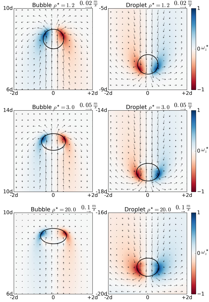
Figure 1: Comparison of equivalent bubble-droplet pairs for density ratio \rho^* = 1.2, 3 & 20 , shown along with the normalized vorticity field \omega_z^* = \omega_z/|\omega_z|_{\max} at steady state. In these cases, the bubble is seen to deform more than the droplet, while the droplet generates more intense and longer trailing vorticity fields. As the density ratio gets farther from unity, the bubble-droplet pair begins to drastically differ. These results are obtained from simulations performed in OpenFOAM in 2D.
