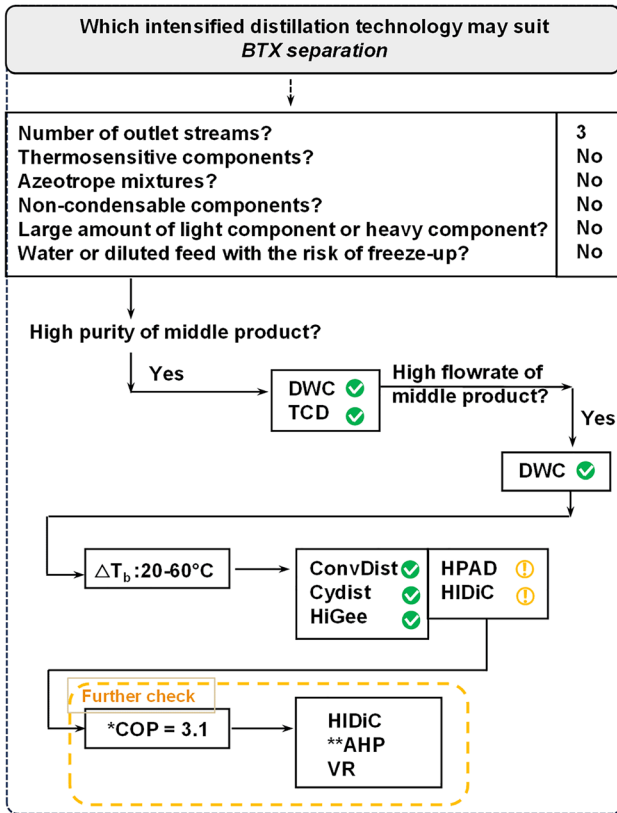
Figure 8: Case study on the benzene/toluene/xylene separation. Note: *Assume compressor efficiency 0.7, minimum temperature difference 5 °C, pressure drop 50 kPa. **AHP, absorption heat pump; VR, vapor recompression.
