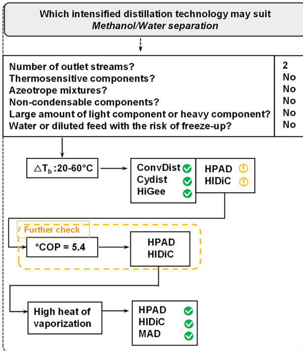
Figure 5: Case study on the methanol/water separation.
