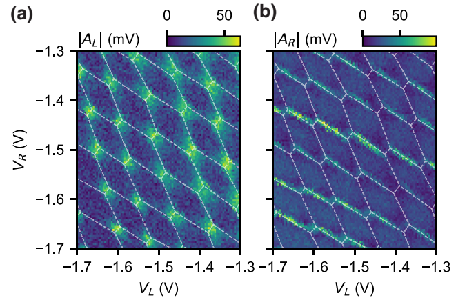
FIG. 4. Charge stability diagram measured using multiplexed gate-based readout in the double dot regime. (a),(b) Amplitude response of the resonators coupled to the two rightmost quantum dots. Readout power in the feedline is -105 \text{ dBm} per multiplexed resonator with an integration time of 3 \mu\text{s} . The dimensions of this dataset are 101 \times 101 points yielding a total integration time of 30 ms excluding overhead from gate settling time, set by low-pass filters on the gate wiring. The dashed lines are guides to the eye delineating the different charge configurations of the double dot and are identical in (a) and (b).
