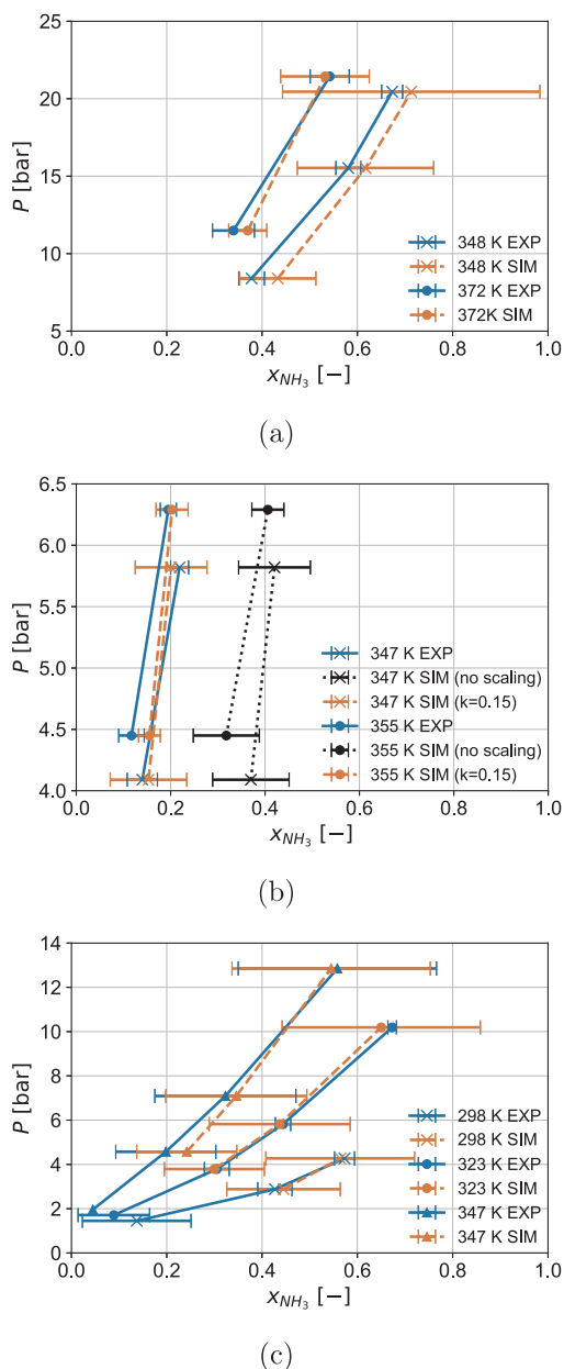
Fig. 2. Comparison between the simulated (SIM) and experimental (EXP) VLE data [10,11] with error bars for the working pairs: (a) \text{NH}_3 /[emim][SCN], (b) \text{NH}_3 /[bmim][BF 4 ] and (c) \text{NH}_3 /[emim][Tf 2 N]. The shown error bars of the simulated data represent the 95% confidence interval.
