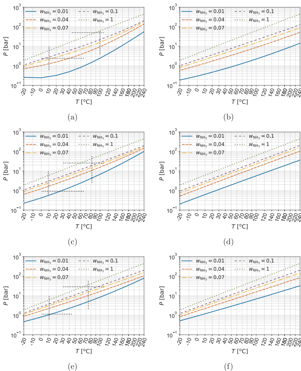
Fig. 11. Comparison of the vapor pressure curves generated only using the experimental VLE data (EXP) and the ones together using the experimental and simulated VLE data (SIM) for the studied NH 3 /IL working pairs: (a) NH 3 /[emim][SCN] pair (EXP [11]), (b) NH 3 /[emim][SCN] pair (EXP [11] + SIM) (c) NH 3 /[bmim][BF 4 ] pair (EXP [10]), (d) NH 3 /[bmim][BF 4 ] pair (EXP [10] + SIM), (e) NH 3 /[emim][Tf 2 N] pair (EXP [10]), (f) NH 3 /[emim][Tf 2 N] pair (EXP [10] + SIM). Vertical and horizontal dashed lines represent temperature and pressure boundaries of EXP data.
