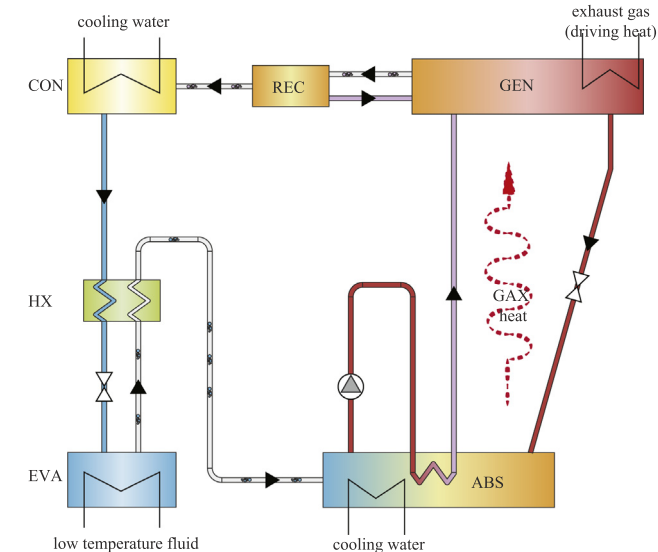
Fig. 7. Schematic diagram of a standard \text{NH}_3/\text{H}_2\text{O} GAX system [8]. The main feature of the GAX cycle is that the final stages of its ABS have higher temperatures than the flow in the first stages of the GEN. The heat from the ABS can be recycled to heat up those stages in the GEN. The weak \text{NH}_3/\text{H}_2\text{O} solutions absorb \text{NH}_3 vapors from the EVA and experience an internal heat recycling in the ABS before they are pumped into the GEN. Vapors leaving the GEN are mixtures of \text{NH}_3/\text{H}_2\text{O} , which are purified in the rectifier (REC). The \text{NH}_3 vapors then experience the similar process as the DE-VAR cycle for generating cooling effects.
