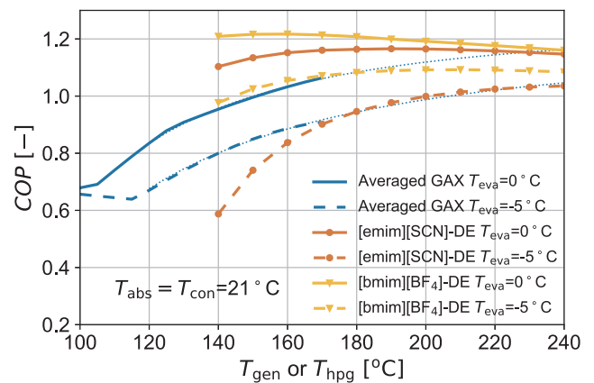
Fig. 15. Comparison of the performance of the DE-VAR with working pairs NH 3 /[bmim][BF 4 ], NH 3 /[emim][SCN] and the NH 3 /H 2 O GAX cycle at condition T_{abs} = T_{con} = 21\text{ }^{\circ}\text{C} . Smooth curves indicate the GAX performance and the dotted curves are extrapolations of their trend lines. The solid curves denote the performance of cooling at T_{eva} = 0\text{ }^{\circ}\text{C} and the dashed curves denote the performance of cooling at T_{eva} = -5\text{ }^{\circ}\text{C} .
