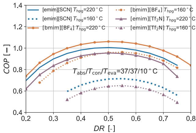
Fig. 12. Influence of the distribution ratio on the coefficient of performance of the DE-VAR with working pair NH 3 /[emim][SCN], NH 3 /[bmim][BF 4 ] and NH 3 /[emim][Tf 2 N]. The performance is calculated at the conditions T_{hpg} are 220 or 160 °C, and T_{abs}/T_{con}/T_{eva} are kept constant at 37/37/10 °C.
