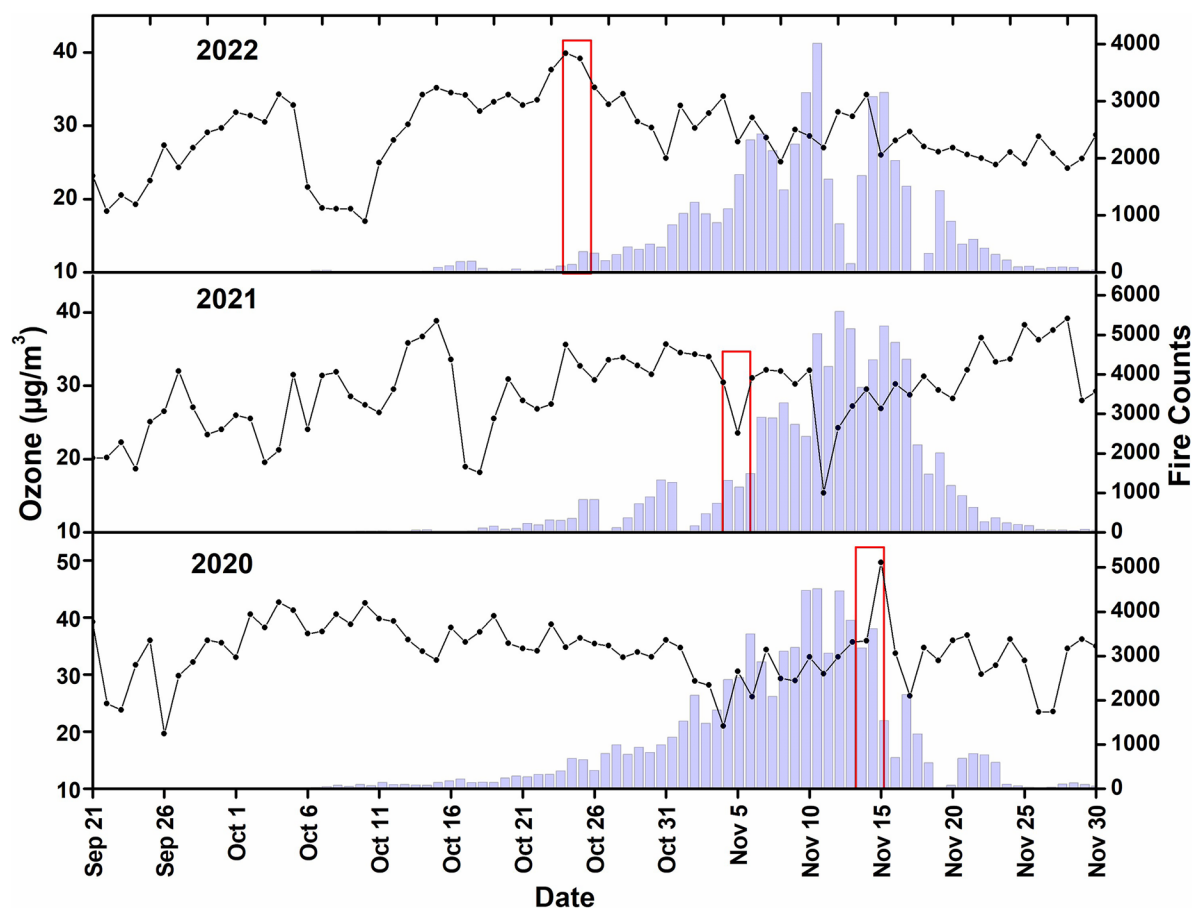
Fig. 11 Graph showing day-to-day variation in number of fire count and corresponding changes in O_3 concentration. Red-coloured rectangle represents the Diwali time in respective years
