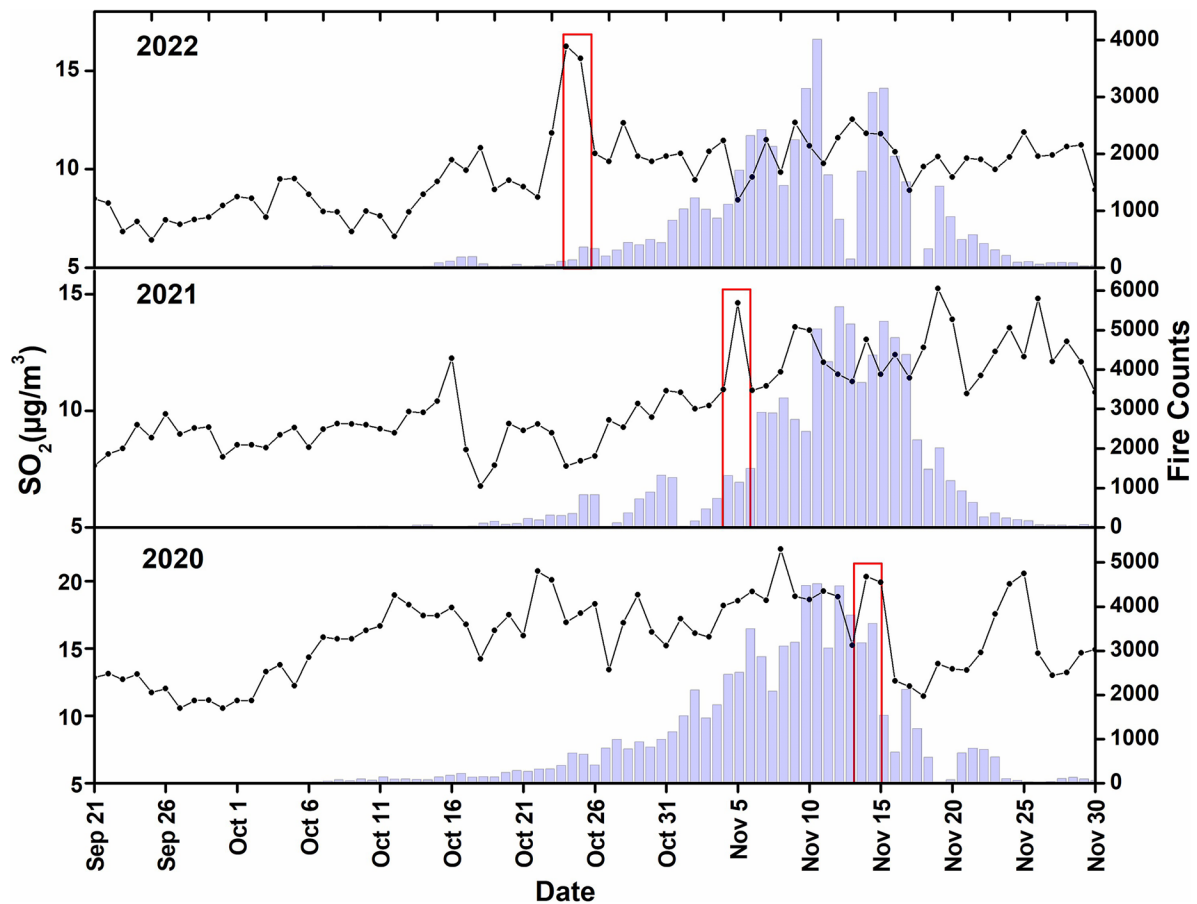
Fig. 9 Graph showing day-to-day variation in number of fire count and corresponding changes in \text{SO}_2 concentration. Red-coloured rectangle represents the Diwali time in respective years
