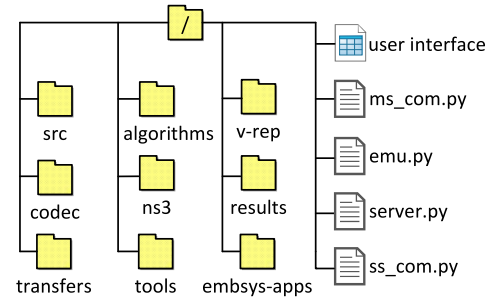
Figure 6. Testbed run-directory.
