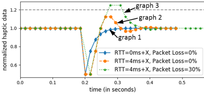
Figure 10. Step response for different RTT and packet drop percentages. X represents the component of RTT that is not part of emulation. The change in pressure (1 \rightarrow 0.5) occurs at around 0.2 seconds.
