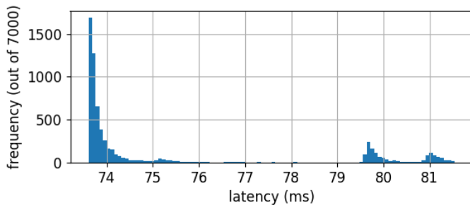
Figure 12. Latency histogram of ping point srv_entry for an intercontinental TCPS setup.
