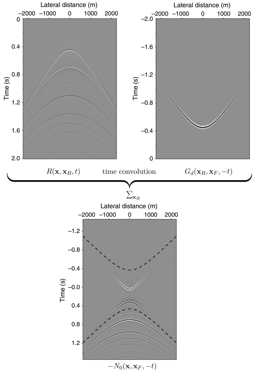
Figure 5. Initialization step to compute f_{1,0}^-(\mathbf{x}, \mathbf{x}_F, t) = -N_0(\mathbf{x}, \mathbf{x}_F, -t) . After applying the time window \theta(\mathbf{x}, \mathbf{x}_F, t) = \theta_t , only events between the dotted lines remain in N_0 . The mute window at t < 0 is applied to mute the wrap-around events of the temporal convolution. This extra window at t < 0 is only a practical solution and is not needed from the theory. Note the difference in the time axes of the three panels: positive for R(t) , negative for G_d(-t) , and negative and positive for N_0(-t) .
