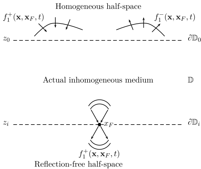
Figure 1. Downgoing and upgoing components of the focusing function f_1 for the 2D wave equation in a truncated medium.
