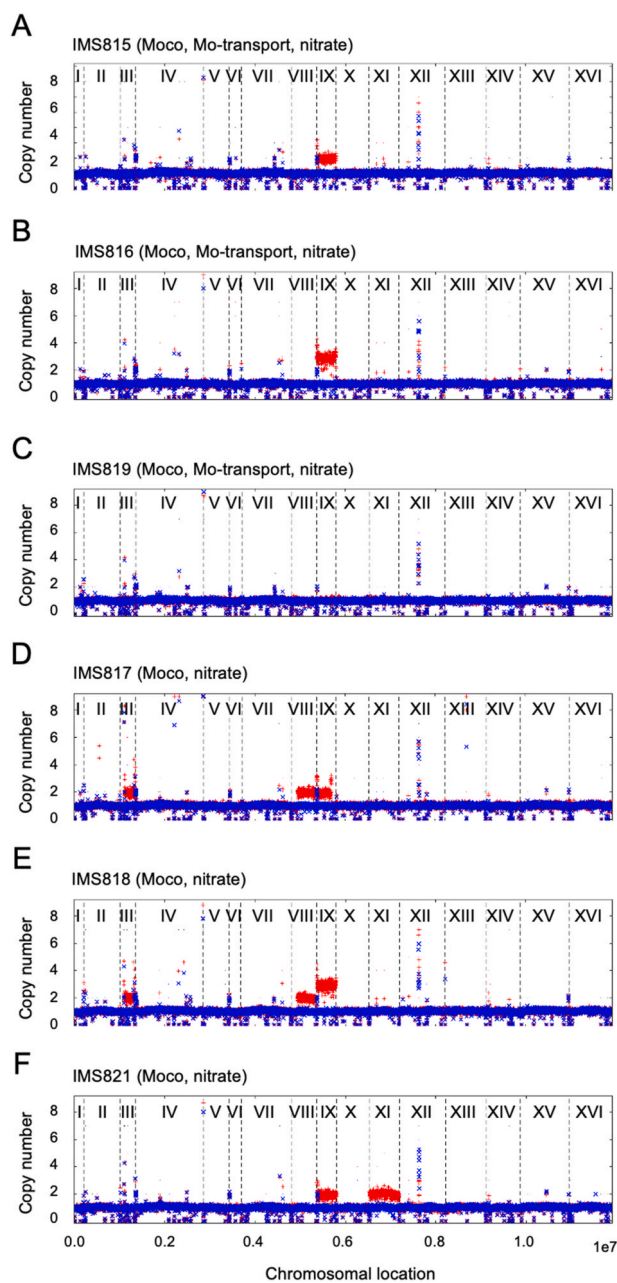
Fig. 4. Chromosomal copy number variations in engineered S. cerevisiae strains evolved for growth in \text{SMD} with 50 mM \text{KNO}_3 as sole nitrogen source. Strains S. cerevisiae IMS815 (A), IMS816 (B) and IMS819 (C) were evolved starting from strain IMX1781 (Moco, Mo-transport, nitrate) while strains IMS817 (D), IMS818 (E) and IMS821 (F) were evolved starting from strain IMX1782 (Moco, nitrate). Copy numbers of chromosomes and chromosomal regions were calculated from sequence data with the Magnolia algorithm (Nijkamp et al., 2012). Results for the parental unevolved strain and the evolved isolate are shown in blue and red, respectively. Individual chromosomes are indicated by Roman numerals and separated by dashed lines.
