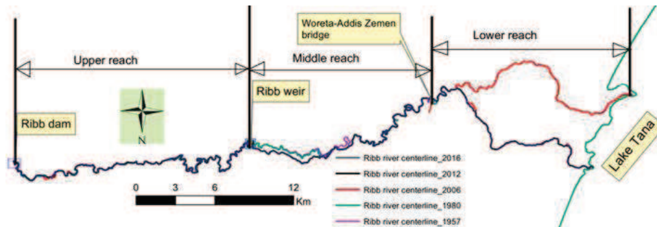
Figure 1. Successive Ribb River channel centrelines.
