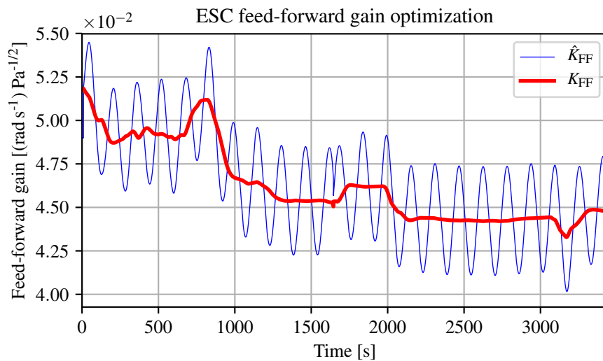
Figure 6: ESC optimization progress of the feed-forward generator speed controller gain K_{\text{FF}} . Convergence to a lower value is observed during the first 2000s, while this value remains near constant in the second half of the process.
