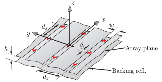
Fig. 8. Doubly periodic connected array of slots radiating in the presence of backing reflector.
