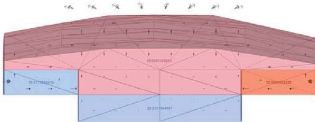
Figure 8 West elevation, thermal and airflow patterns for design case 1.
