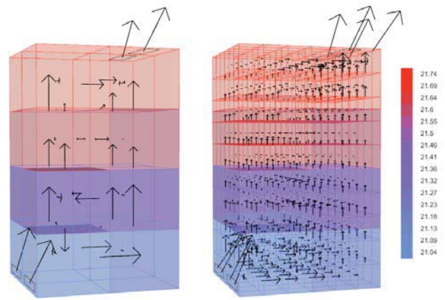
Figure 1. Left: Thermal zones colored according to temperature values, arrows showing airflow directions and relative amount of air in between neighboring thermal zones. Right: Airflow zones colored according to temperature values, arrows showing airflow directions and relative amount of air in between neighboring airflow zones.
