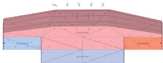
Figure 9 West elevation, thermal and airflow patterns for design case 1.
