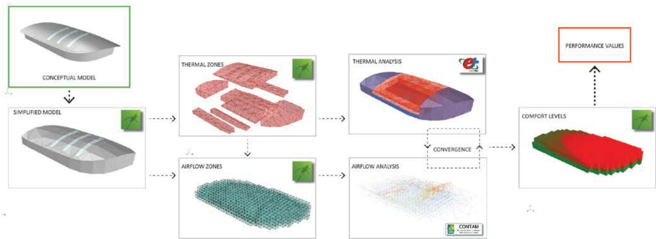
Figure 2. Computational system framework for the rapid assessment of comfort levels based on temperature and airflow predictions, using CONTAM and E+ simulation software integrated with Grasshopper plugin for Rhino.
