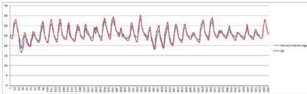
Figure 4. Average indoor temperature fluctuation for the simulated period (May). Red: DB results. Blue: Proposed process results.
