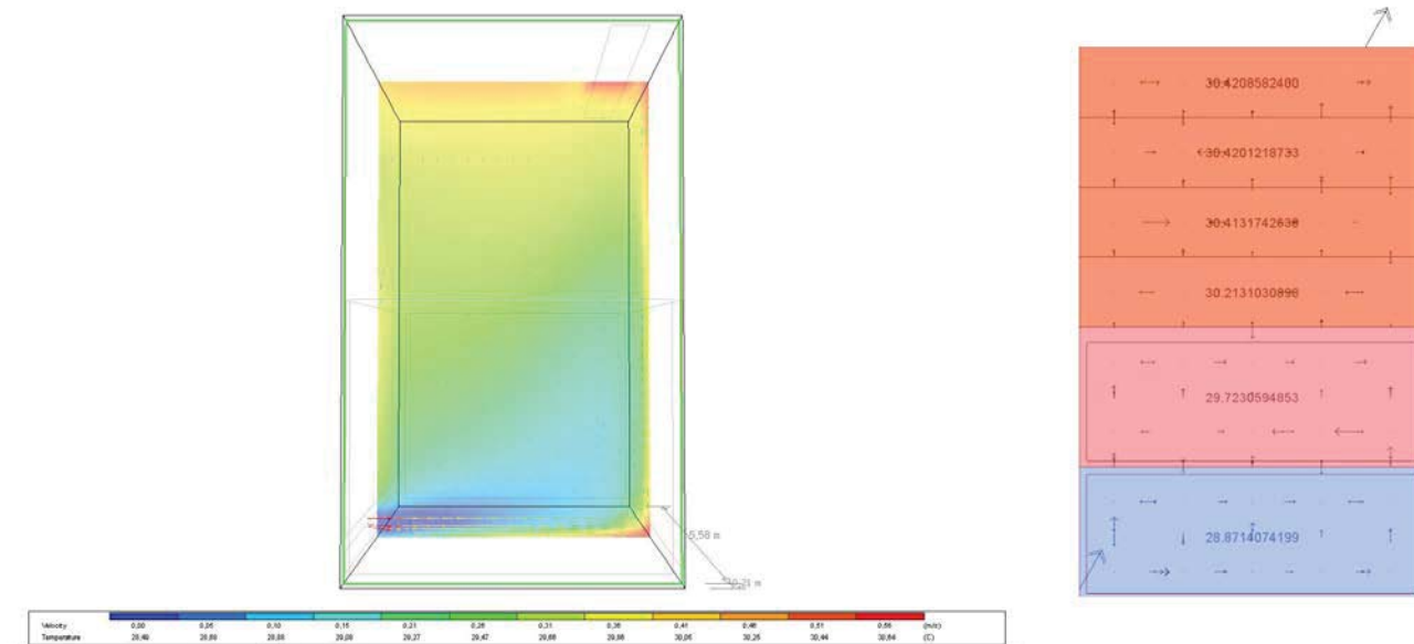
Figure 3. Left: CFD analysis done in the DB software. Right: Zone temperatures and airflow distribution with the developed approach.
