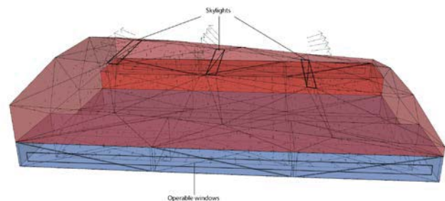
Figure 6 Ventilation openings on the side facades and roof.
