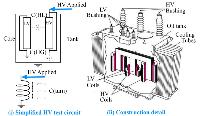
FIGURE 6. MV distribution Transformer [23].
