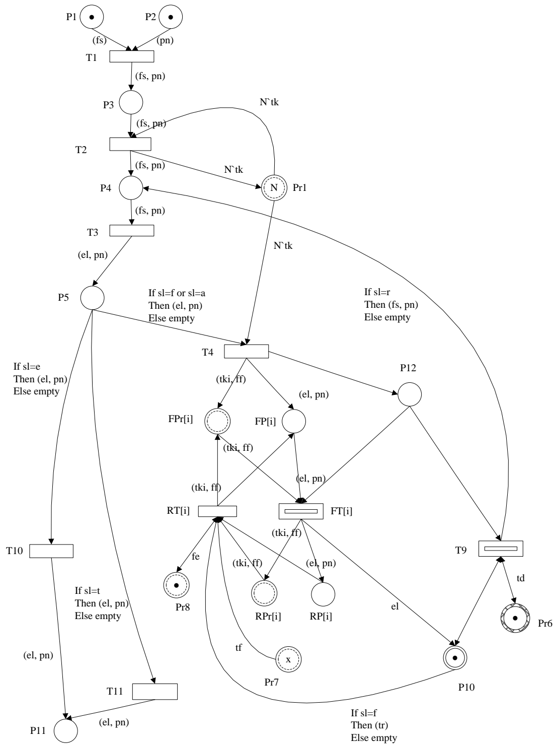
Fig. 4 Type 1 model (without queuing refilling system)
