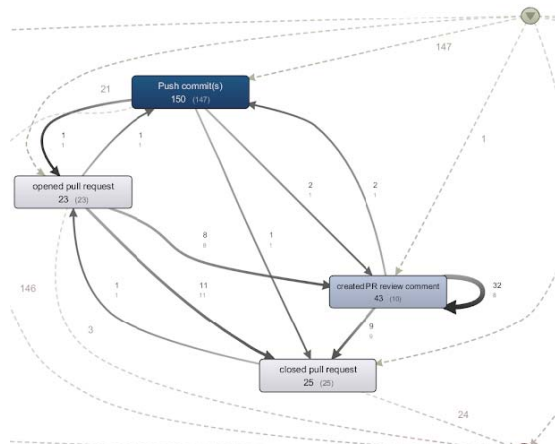
Fig. 1. Excerpt from the Apache Camel process map.
