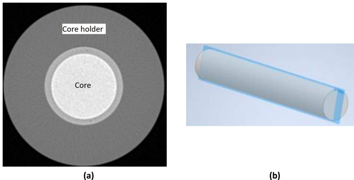
Figure 14: (a) Example of a CT slice showing a cross section of the core inside the PEEK core holder (b) vertical plane through center of core showing where results are plotted
