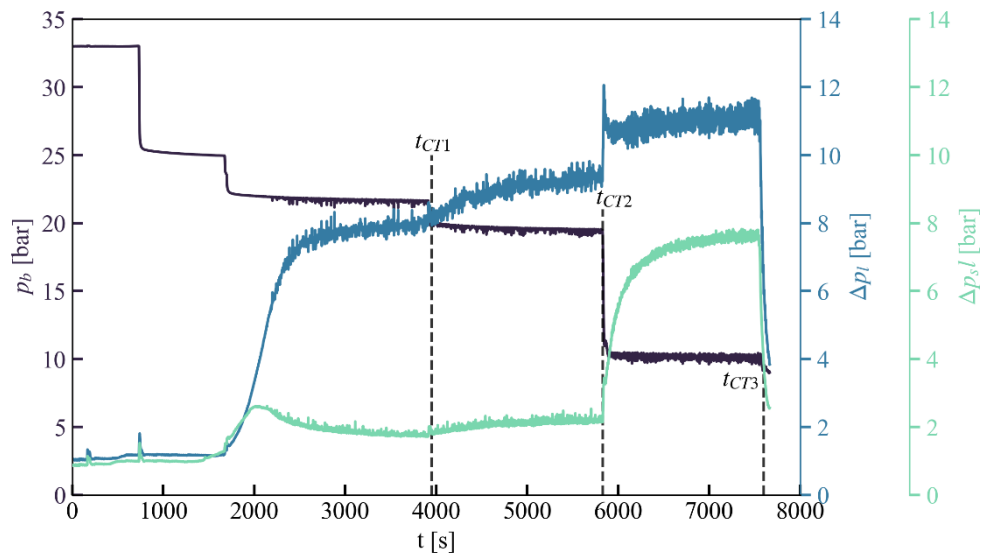
Figure 18: Backpressure ( p_b ) along with pressure drop in the last section ( \Delta p_l ) and second to last section of the core ( \Delta p_{sl} ) using a CO 2 concentration of 0.9 mol/L. CT scans are taken at t = t_{CT1} , t_{CT2} and t_{CT3}
