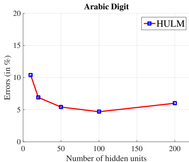
Fig. 6: Generalization error (in %) of the hidden-unit logistic model on the Arabic speech data set as a function of the number of hidden units.
