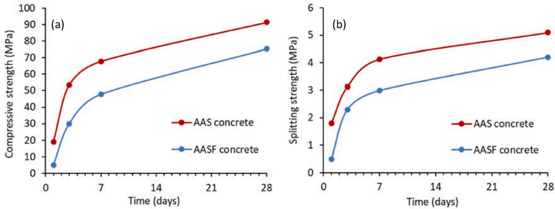
Fig. 2. Measured compressive (a) and splitting tensile (b) strength of AAS and AASF concrete.
