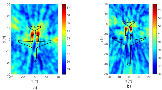
FIG. 7. Beamforming plots for high frequency band: (a) F70 (b) MD81 25 .
