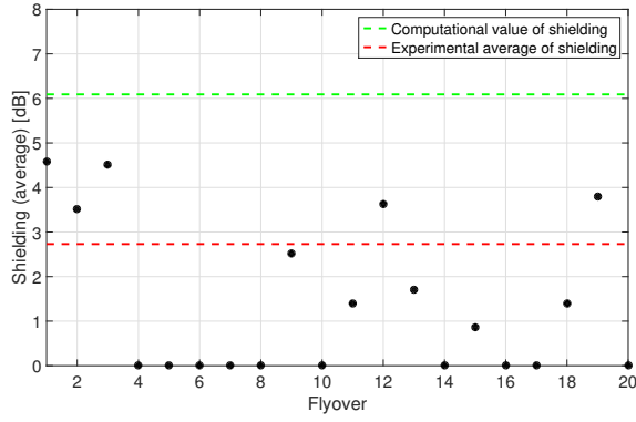
FIG. 17. Measured and predicted value of noise shielding found for different flyover measurements of the F70. The dots indicate the shielding for the 20 flyovers and the red dashed line - - - indicates the average value of the flyovers with noise shielding. The green dashed line - - - is the predicted value of shielding.
