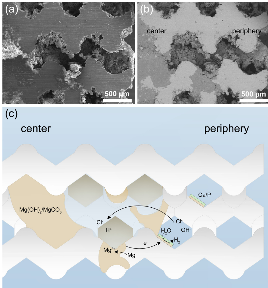
Fig. 7. Macroscopic degradation behavior of scaffolds on the cross-section after 7-day immersion: (a) SEM image, (b) BSE image and (c) schematic illustration of degradation at the center of the WE43 scaffolds.
