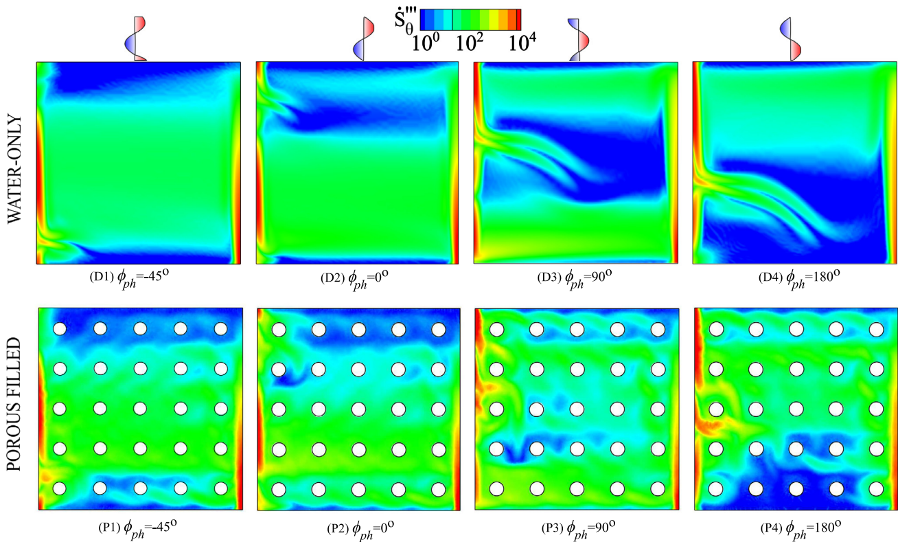
Fig. 13. Entropy generated in the fluid region due to temperature gradient in a characteristic vertical plane at X/L = 0.41 in a water-only (top row) and porous media filled (bottom row) cavity, with the left wall having sinusoidal temperature distribution with amplitude \theta_i^{amp} = 1 and varying phase angle \Phi_{ph} , at Ra_f = 10^7 .
