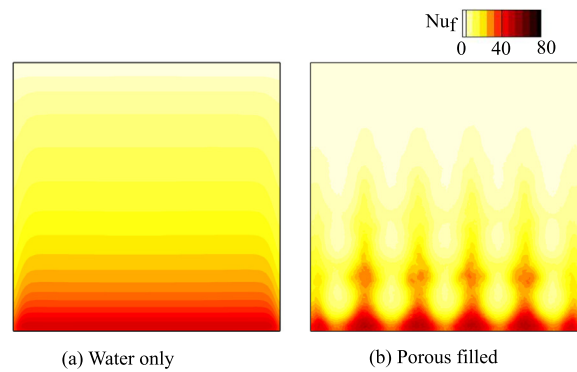
Fig. 4. Nusselt number contour on the right wall in a water-only (a) and porous media filled (b) cavity, with constant temperature of \theta_l = 0 and \theta_r = 1 , at Ra_f = 10^7 . The contours are represented using a linear scale with 30 contour levels.
