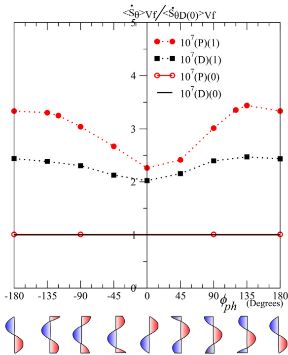
Fig. 14. Variation of non-dimensional entropy generation of fluid due to temperature gradient with phase angle at Ra_f = 10^7 , with SWT ( \theta_i^{amp} = 1 ) and CWT ( \theta_i^{amp} = 0 ) in a water-only (D) and porous media filled (P) cavity.
