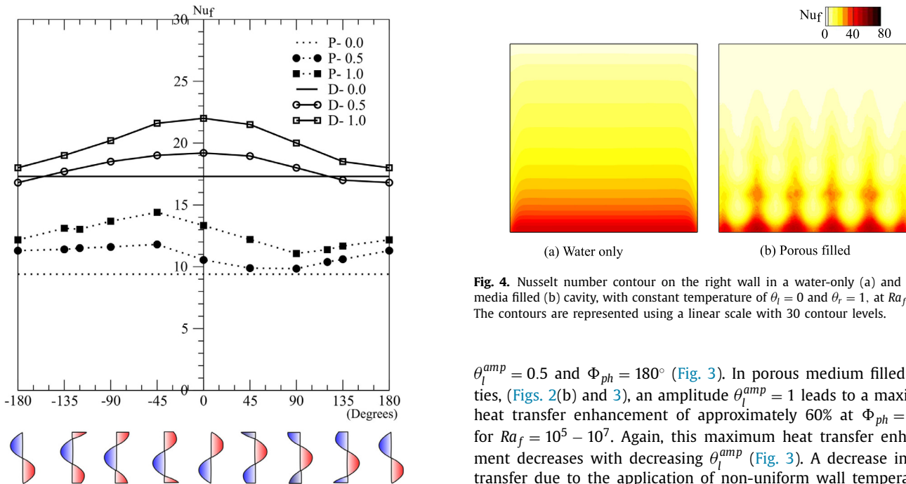
Fig. 3. Variation of wall-averaged Nusselt number with phase angle at Ra_f = 10^7 and different amplitudes, \theta_l^{amp} (0, 0.5, 1) of cold wall temperature variation in a differentially heated water-only cavity (D) and porous media filled-cavity (P).
