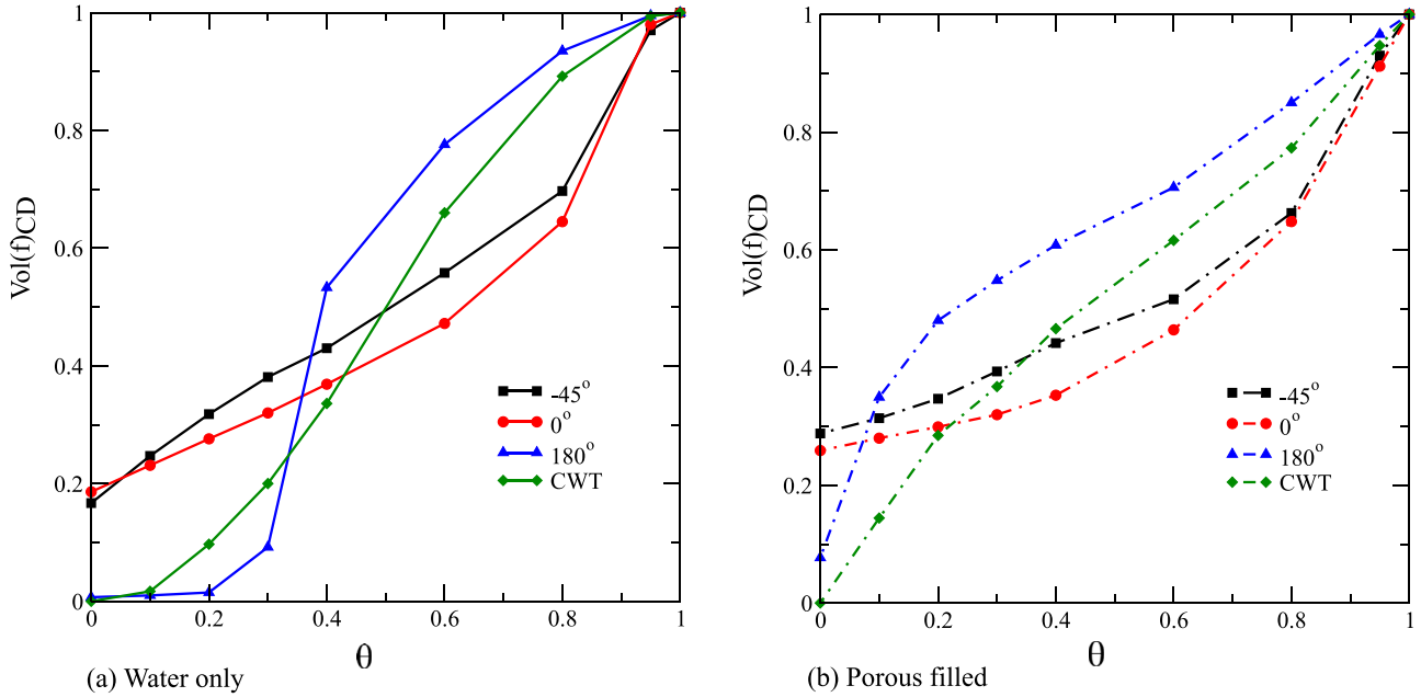
Fig. 11. Cumulative distribution (discrete) of the fraction of fluid volume where \theta \leq \zeta\theta_{max} , in water-only (a) and porous media filled (b) cavities, with the left wall having a sinusoidal temperature distribution with amplitude \theta_i^{amp} = 1 at \phi_{ph} = -45^\circ (black), \phi_{ph} = 0^\circ (red), \phi_{ph} = 180^\circ (blue) at Ra_f = 10^7 . The results are compared with the respective cavities at constant wall temperature (green). (For interpretation of the references to color in this figure legend, the reader is referred to the web version of this article.)
