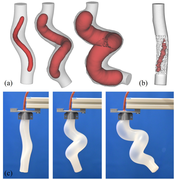
Fig. 7: Simulation results for a soft robot with twisting deformation under actuation. (a) By progressively remodeling the chamber region \mathcal{M}_c (shows in red), our method can generate the results that mimic the physical behavior shown in (c) as applying different volume-based actuation parameters (from left to right: \alpha = 5, 28 , and 115). (b) Directly applying a large actuation parameter \alpha = 28 leads to an unrealistic result in simulation.
