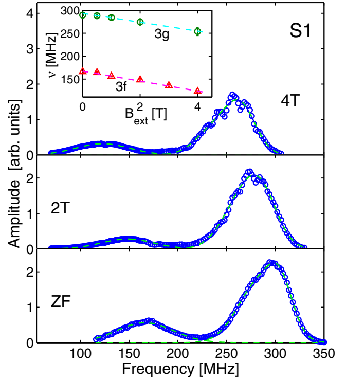
FIG. 4. ^{55}\text{Mn} NMR spectra of sample S1 at T = 5 \text{ K} , in zero and in perturbing applied fields. Inset: Mean positions of the 3f and 3g lines as a function of the external field. The dashed lines are fits to Eq. (1).
