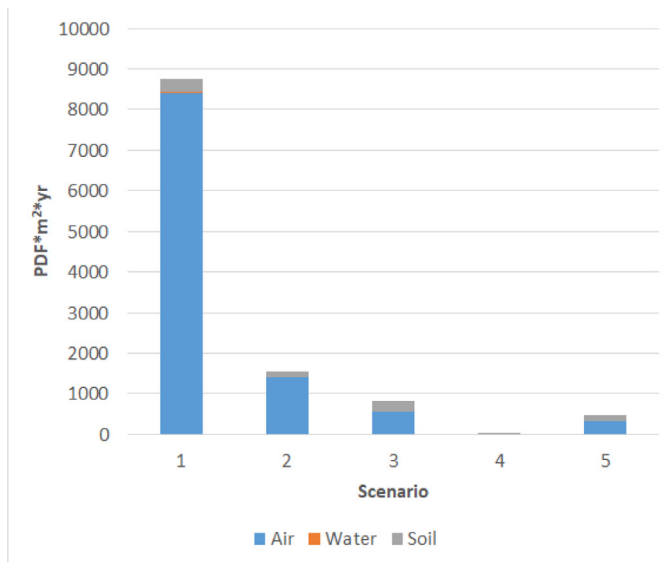
Fig. 6. Profile of emissions impacting ecosystem quality across scenarios.
