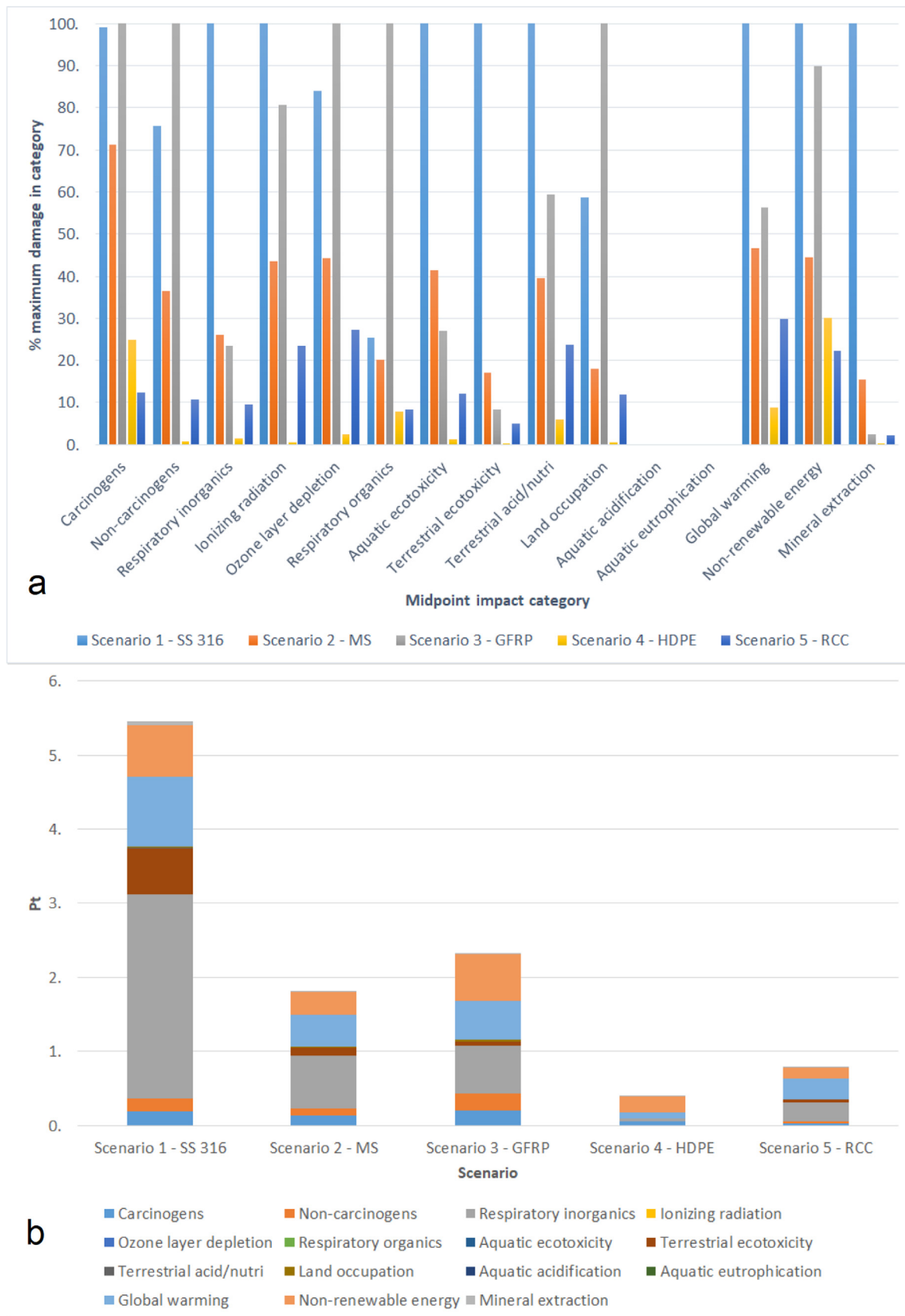
Fig. 2. Impact profiles across scenarios with regards to midpoint categories. (a.) Damage assessment by category. (b.) Single score.
