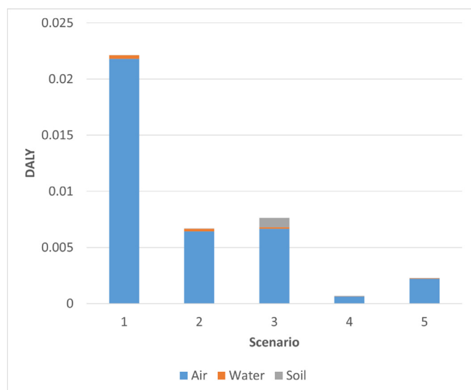
Fig. 4. Profile of emissions impacting to human health across scenarios.
