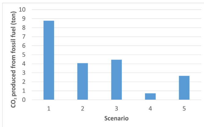
Fig. 7. Relative CO 2 profiles of each scenario due to fossil fuel consumption.
