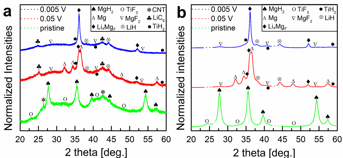
Fig. 3. XRD patterns of the \text{MgH}_2 electrode at different stages: pristine, lithiated to 0.05 V and 0.005 V, respectively. (a), experimental data; (b), Refined XRD patterns after subtraction of background; (The 2 theta ranges of carbon and Li-C alloy has been subtracted since it is out of the scope of this work. Details on the refinement are displayed in Fig. S6 .) Here the electrode is a pressed pellet ( \sim 70 \mu\text{m} in thickness), instead of a slurry based electrode, in order to avoid the strong Bragg reflections from the Cu current collector and to produce XRD patterns with a higher signal-to-noise ratio.
