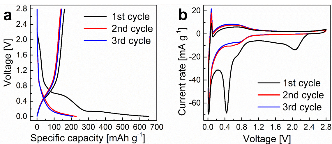
Fig. 4. (a), Voltage profiles at 0.05 C and (b), Cyclic voltammograms (scan rate: 0.02 mV s -1 ) of the MgH 2 -TiF 3 electrode tested in a Na ion half-cell.
