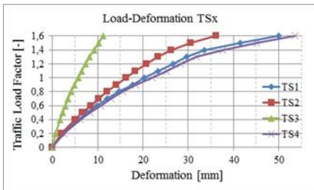
Figure 10. Load-deformation diagram traffic load cases
