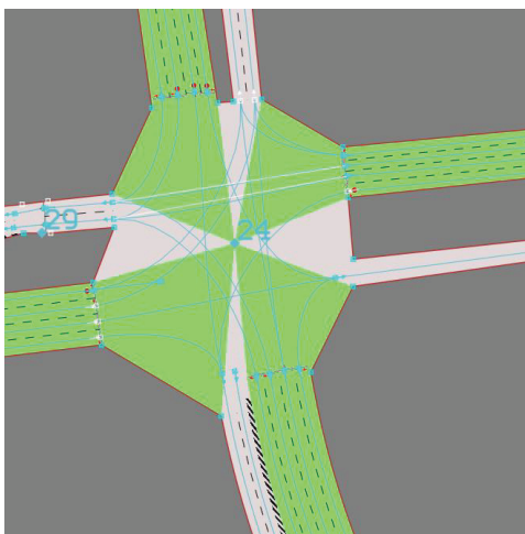
Figure 7.25: Paramics Discovery: entrance links (green) joining at node 24
