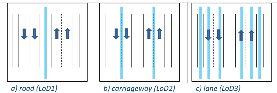
Figure 6.14: proposal for the representation of a motorway (2 * 2 lanes and shoulder) at three levels of detail (blue lines)
