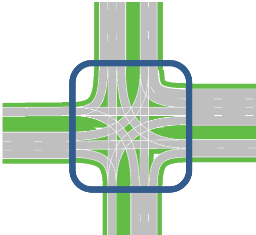
Figure 7.14: the JunctionArea describing the (virtual) lanes enclosed by the blue rectangle (based on work from W. Schakel)
