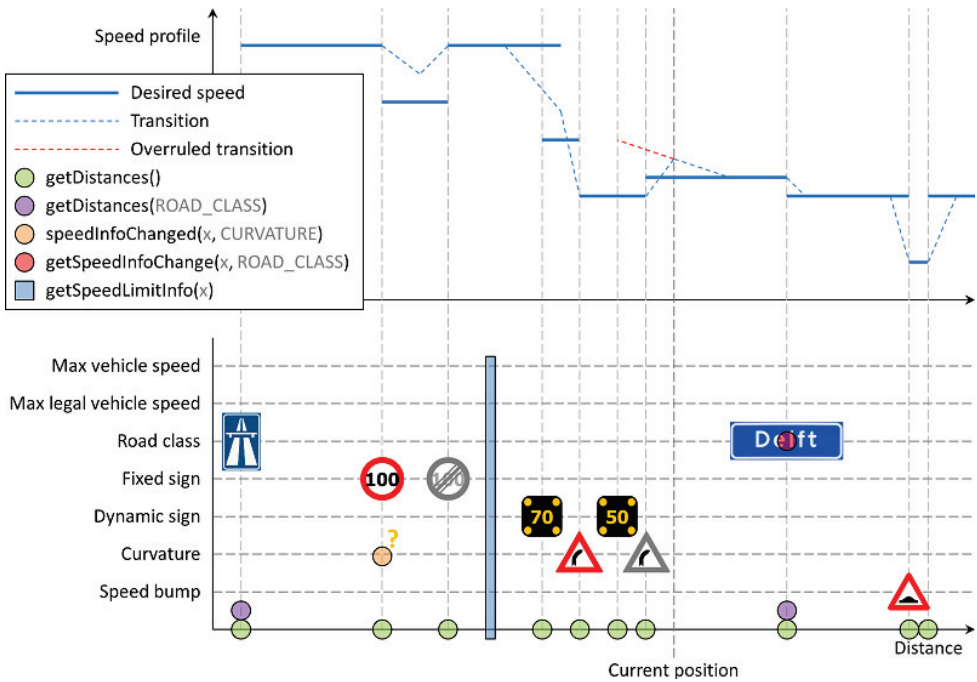
Figure 7.12: Speed profiles in relation to infrastructure (made by W. Schakel 15 )
