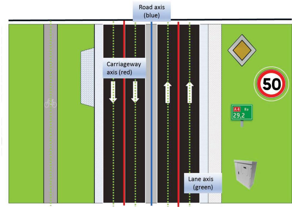
Figure 6.13: Combined representation of a road by lines and spaces (source: Marleen Hovens, CROW)
