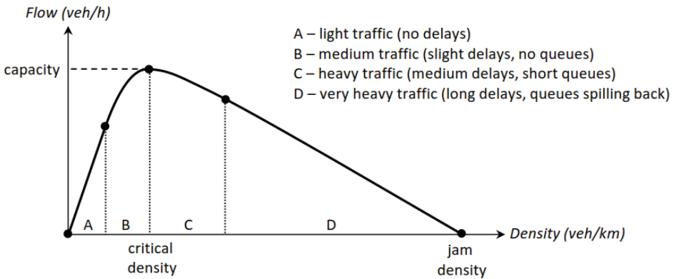
Figure 5.4: fundamental diagram (source: Bliemer, Raadsen et al. (2015) ).
