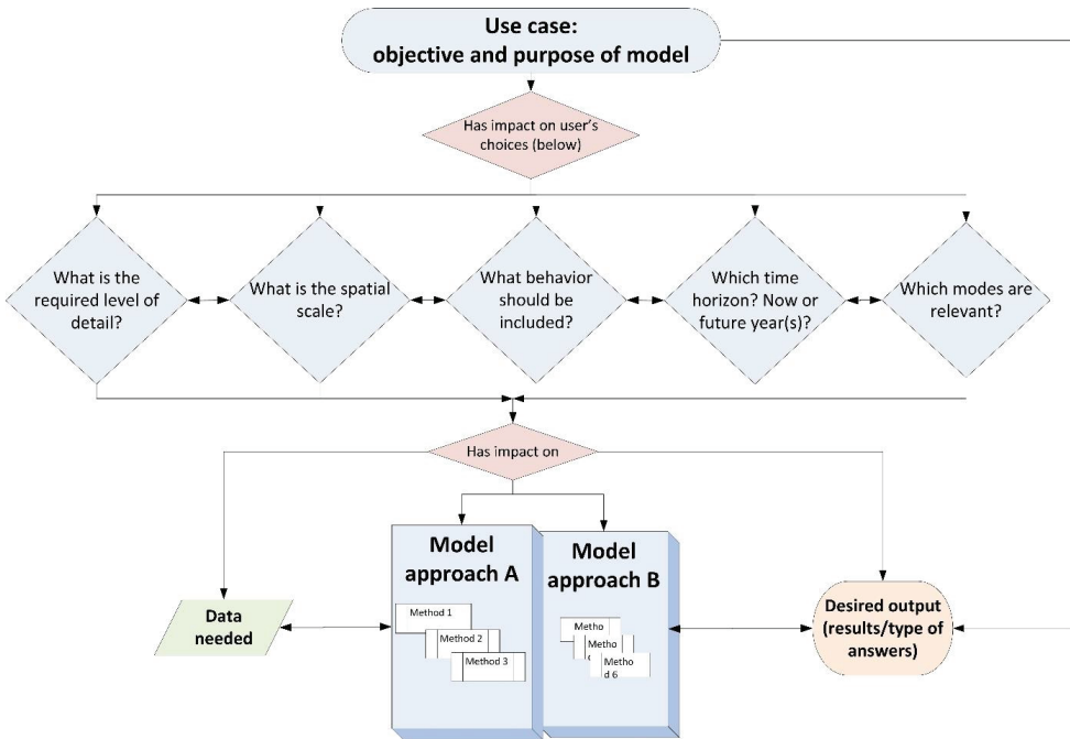
Figure 2.2: the use case, its impact on the phenomena to be modelled, and subsequently the choice for a model approach
