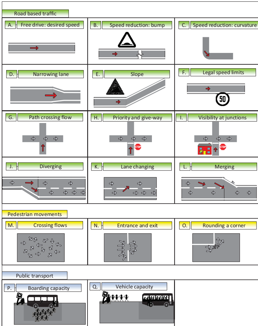
Figure 4.3: overview of typical situations that have an impact on speed and capacity (pedestrian movements based on Duives, Daamen et al. (2013) )
