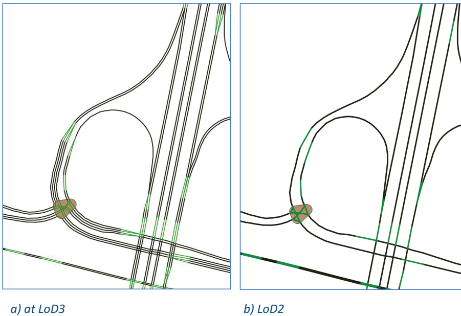
Figure 6.17: example of the representation of a small network by (a) lane and (b) carriageway (by direction)
