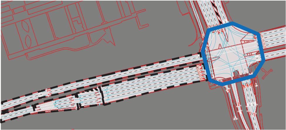
Figure 7.23: Partitioning the road area (see Figure 7.22) into separate spaces that better align with the road network characteristics.
