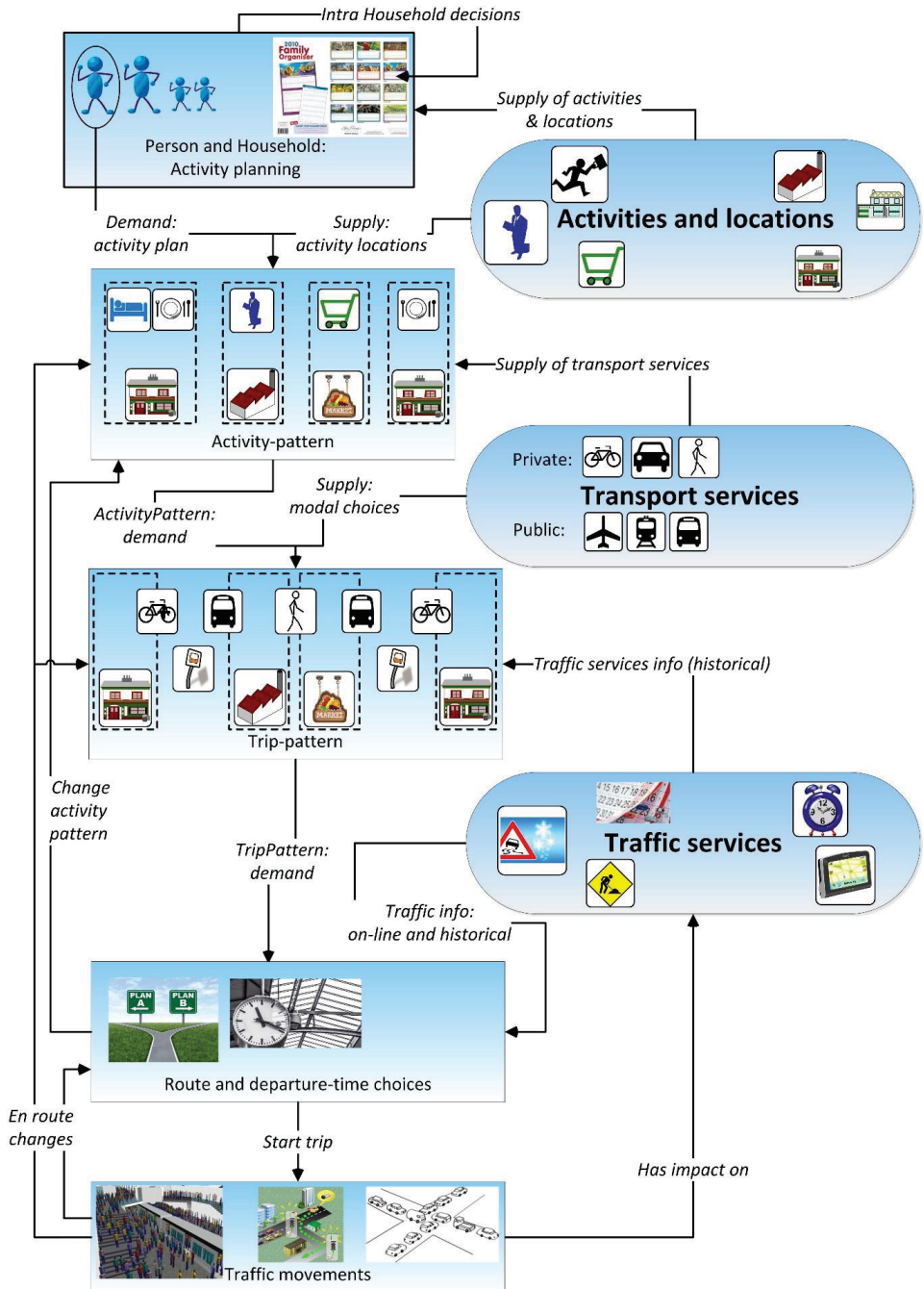
Figure 2.1: Modelling transport & traffic at a person's level
