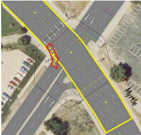
Figure 7.24: Vissim: link (yellow) and connector (red: right turning movement) to another link
