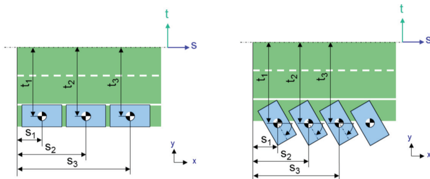
Figure 6.5: Modelling of parking lots in OpenDrive (source: Consortium (2012), Dupuis (2015))
