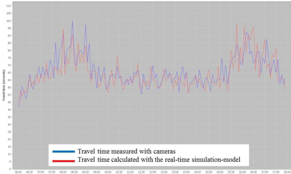
Figure 8.21: Comparison of travel times at the N201 measured with license plate recognition cameras (blue) and the real-time simulation-model (red)
