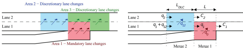
Figure 5.10: transforming discrete lane changes into continuous descriptions (source: Leclercq, Marczyk et al. (2016) )
