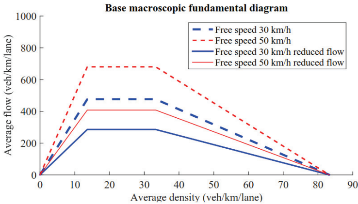
Figure 5.7: base network fundamental diagram (source: Knoop, Tamminga et al. (2016) )
