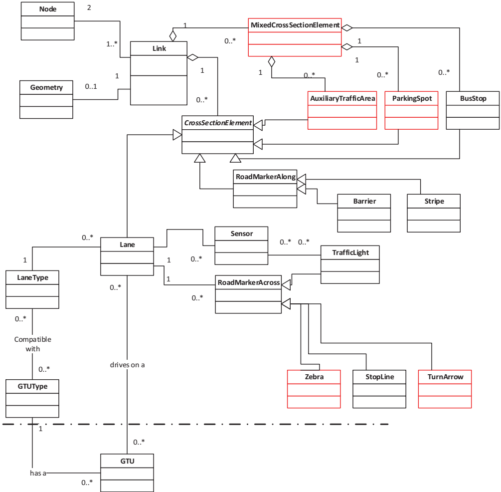
Figure 7.6: Pseudo XML schema of the Link design 14
