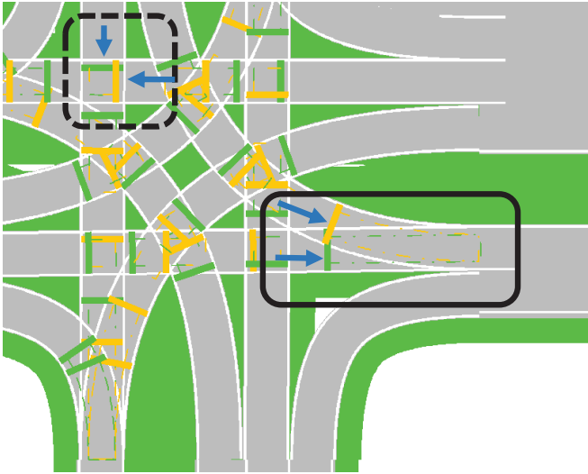
Figure 7.15: priority at conflicting lanes: merging and crossing paths (based on work from W. Schakel)
