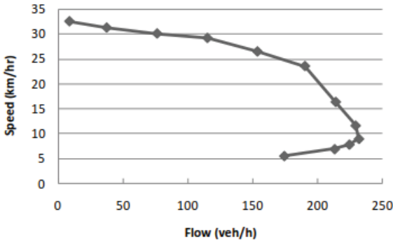
Figure 5.9: Speed-flow relationship based on microsimulation (source: Liu, May et al. (2011))
