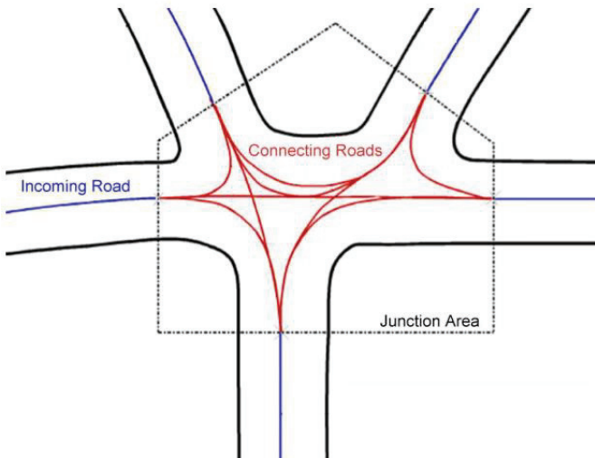
Figure 6.11: junction lay out in OpenDRIVE (source: Dupuis (2015) )
