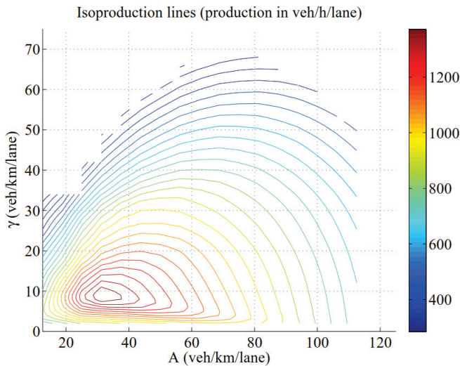
Figure 5.8: Iso-production lines from the generalized macroscopic fundamental diagram (source: Knoop, Hoogendoorn et al. (2013) )
