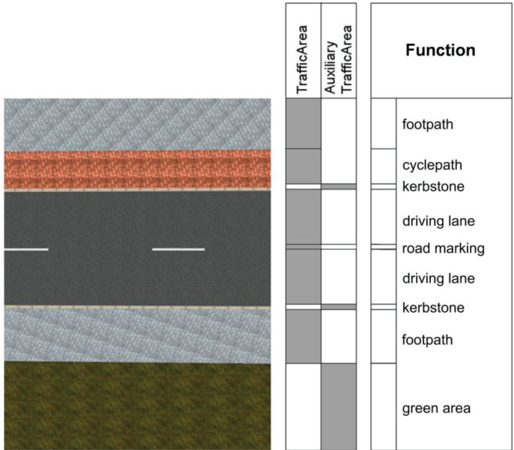
Figure 6.7: example of a Cross Section profile of a road (source: Consortium (2012))
