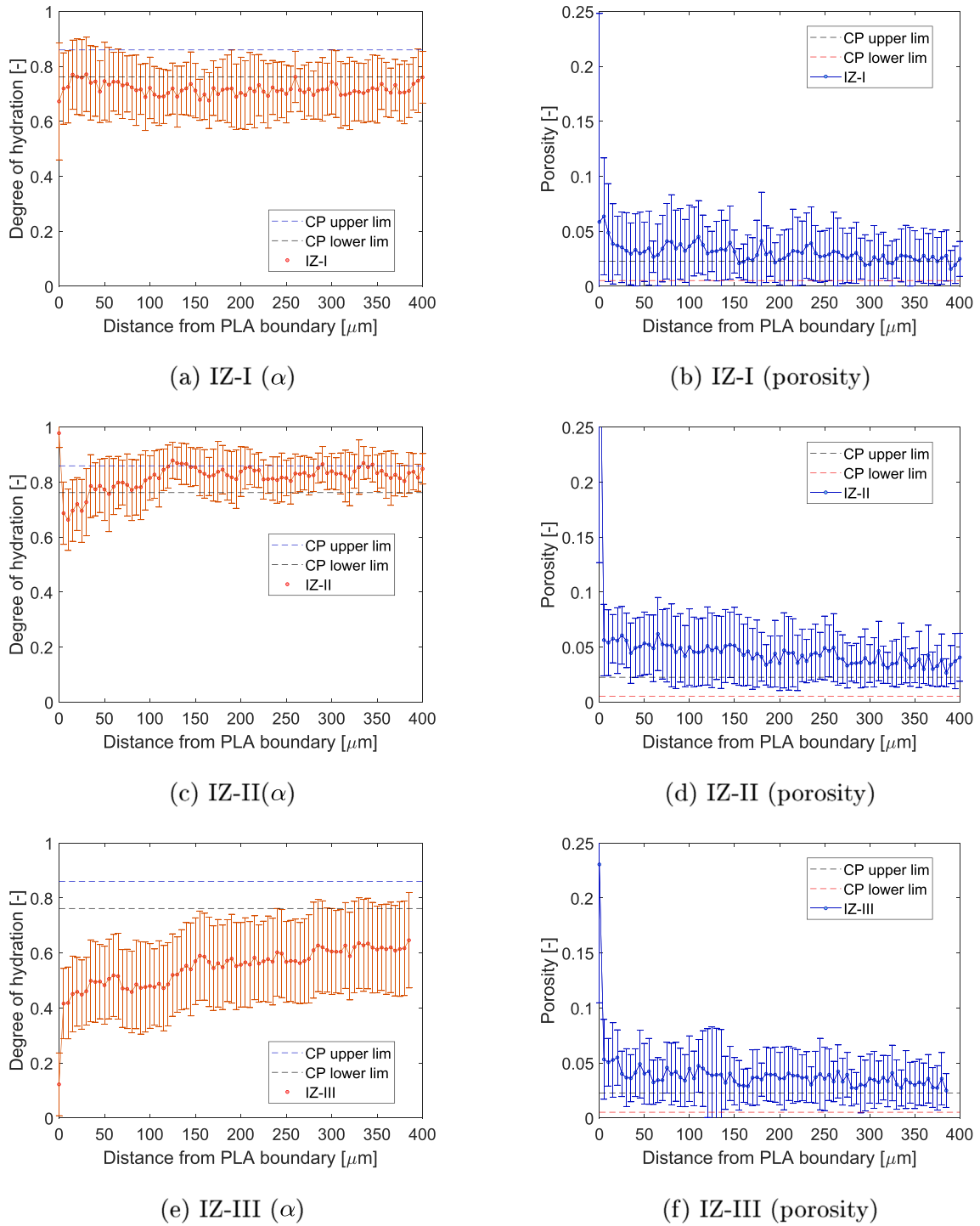
Fig. 6. Degree of hydration profiles from PLA boundary of the IZ of SH-I a), -II c) and -III e) and porosity profiles from PLA boundary of the IZ of SH-I b), -II d) and -III f). The error bars represent the standard deviation among the different micrographs for each position.
