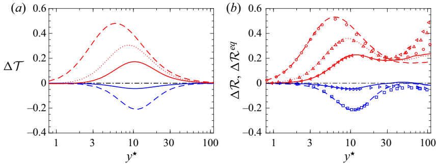
Figure 13. Difference in viscous ( \Delta T ) and turbulent ( \Delta R ) shear stress at x/h = 35 . Symbols in panel (b) show profiles of turbulent shear stress assuming negligible advection (i.e. C_u = 0 ) ( \Delta R^{eq} ).
