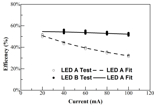
FIGURE 4. Efficiency curves vs. driving current.
