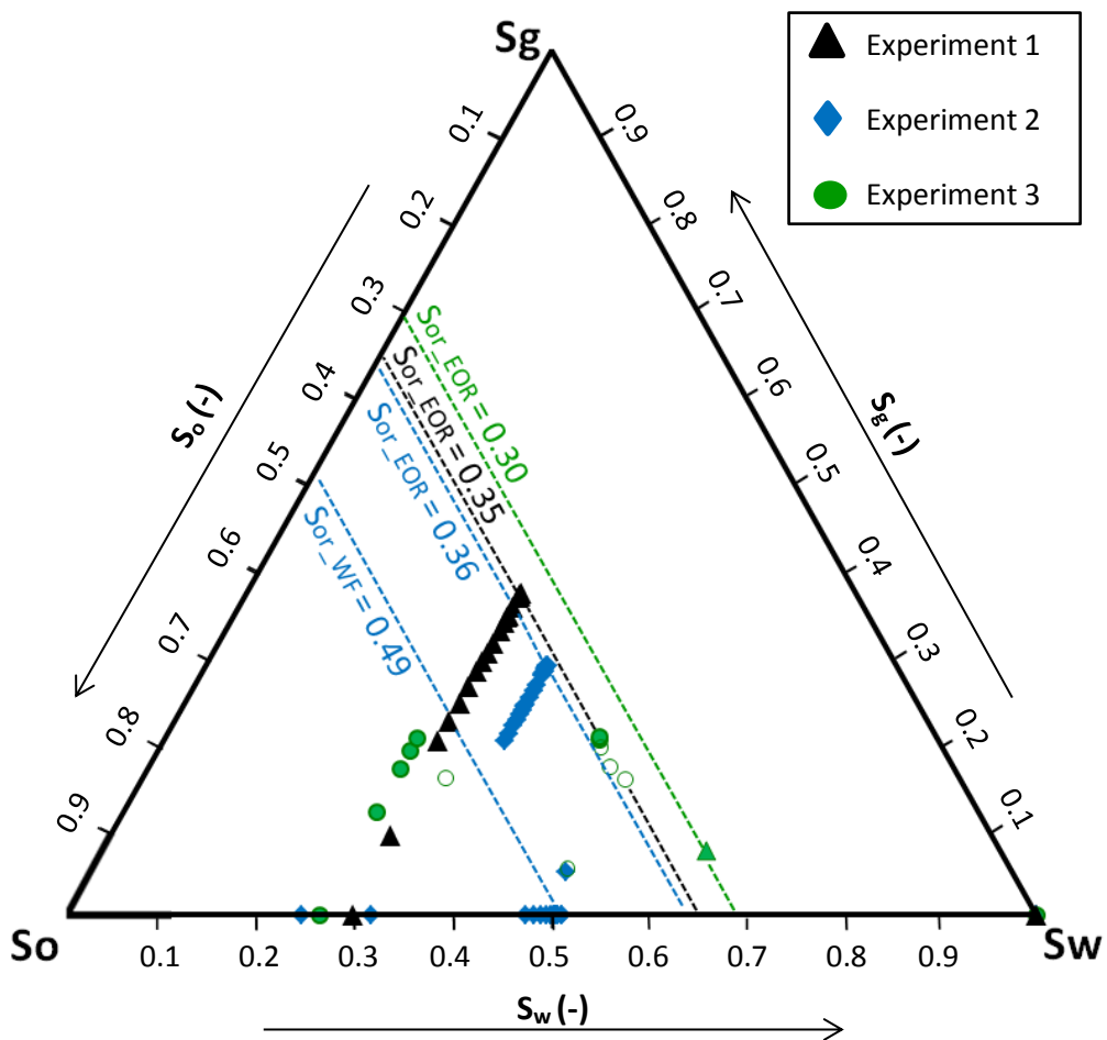
Figure 12: Saturation paths for Exp. 1, Exp. 2 and Exp. 3. S_w , S_o , S_g , S_{or\_WF} and S_{or\_EOR} represent the water, oil, gas, residual oil to waterflood and residual oil to immiscible gas/WAG respectively. Three-phase saturations shown were averaged over the entire core and calculated using material balance calculations. The closed and open circles in Exp. 3 represent the gas and water injection during the first two WAG cycles respectively. The green triangle indicates the saturation distribution after successfully injecting 12 full WAG cycles.
