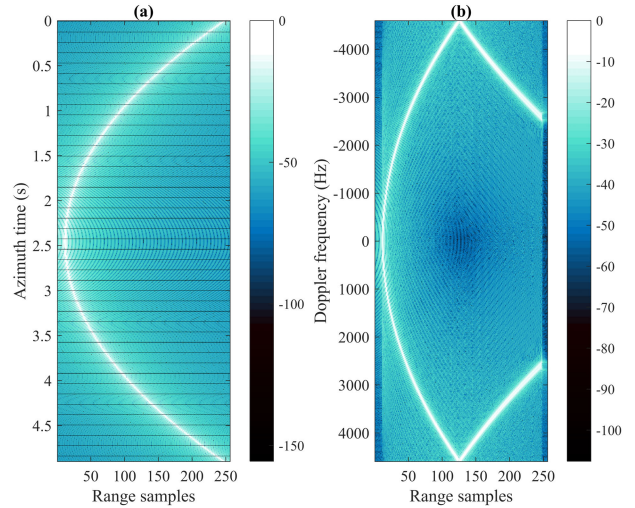
Fig. 3. 2-D power radargram (dB) of a simulated point target for 4.9 s in (a) range/azimuth domain and (b) range/Doppler domain. Due to the limited PRF, we only can process frequencies below \text{PRF}/2 = 4.65 kHz. Frequencies higher than half of the PRF become folded within the limits of the sampled spectrum, appearing as interference in higher ranges.
