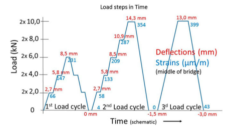
Fig. 22: Three load cycles during the test on 17 August 2018 showing applied load, max strain in middle and maximum measured vertical deflection
