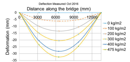
Fig. 17: Results measured LDVT deflections at production facility test 21 October 2016
