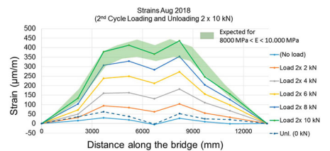
Fig. 24: Second load cycle; results of strains in tension sensors along the bridge (line 2), stepwise loading and unloading to 2 \times 10.0 \text{ kN}
