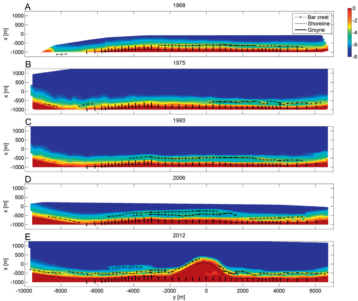
Fig. 5. Five JARKUS surveys including detected sandbars. The shading indicates bed level with respect to the local datum ( \approx mean sea level). Detected bar crests, the shoreline and the locations of rubble-mound groynes are indicated with markers and lines (see legend). The local coordinate system is aligned with the average coastline orientation and has its origin at the tip of the Sand Motor.
